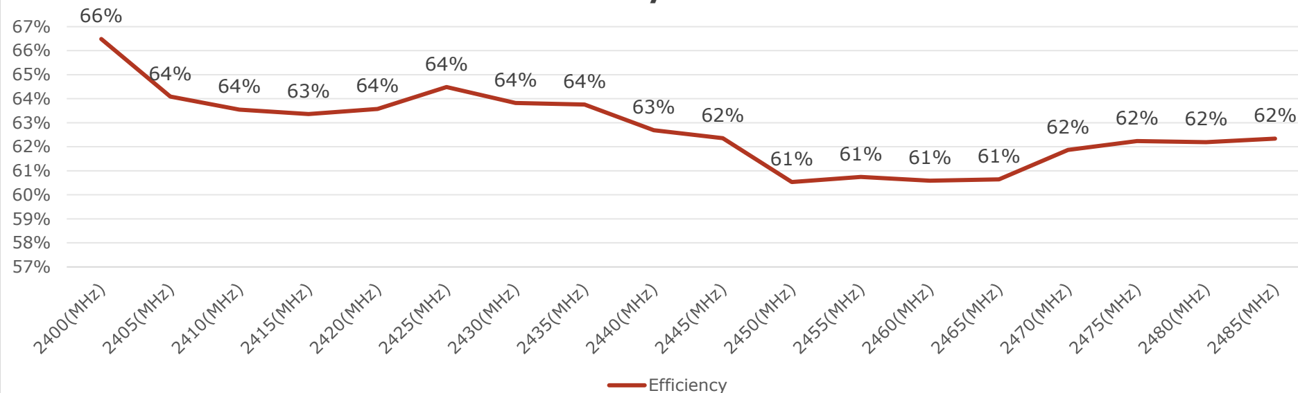
Efficiency of VPH14
