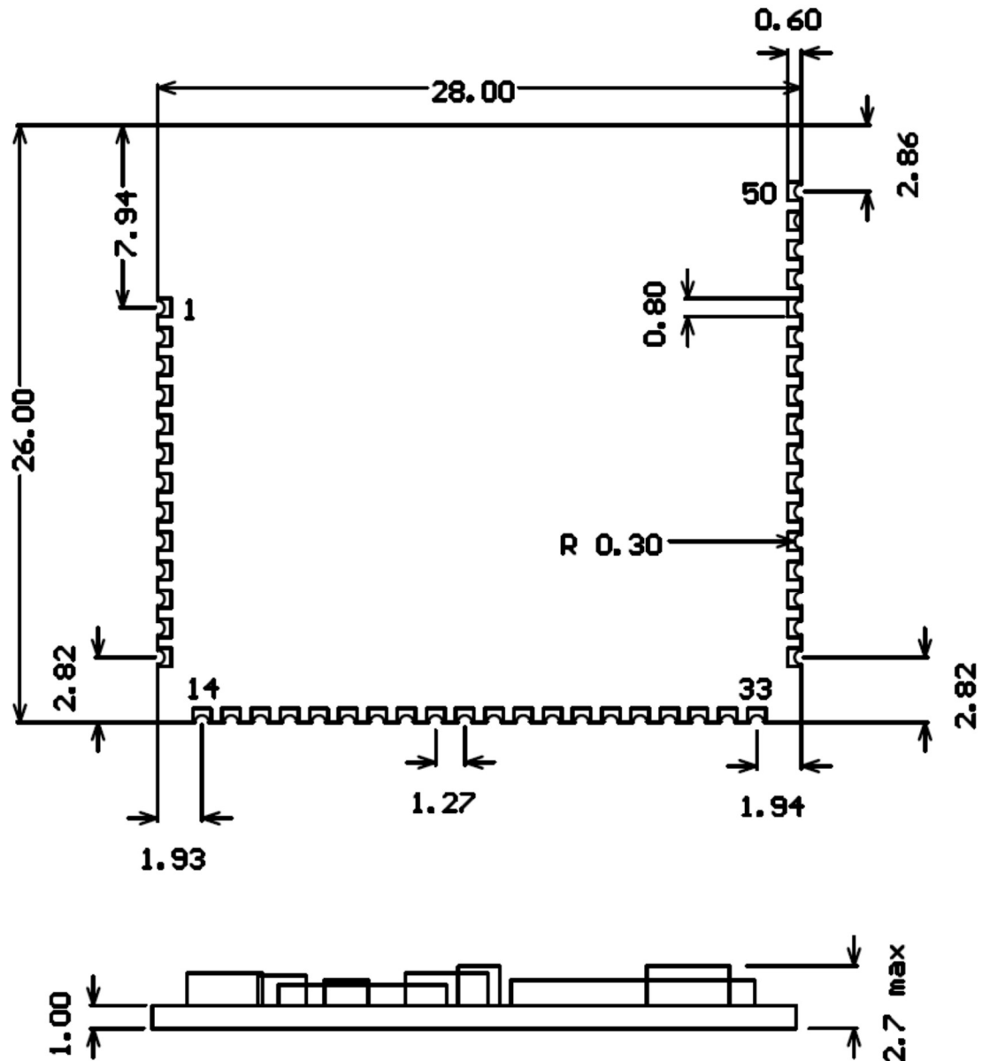
Figure 4 AVT9152 Mechanical Dimensions
