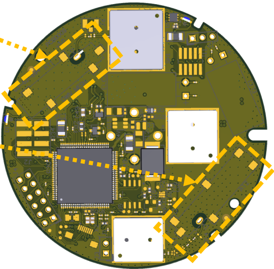
2.4 GHz MESH Transmitter
