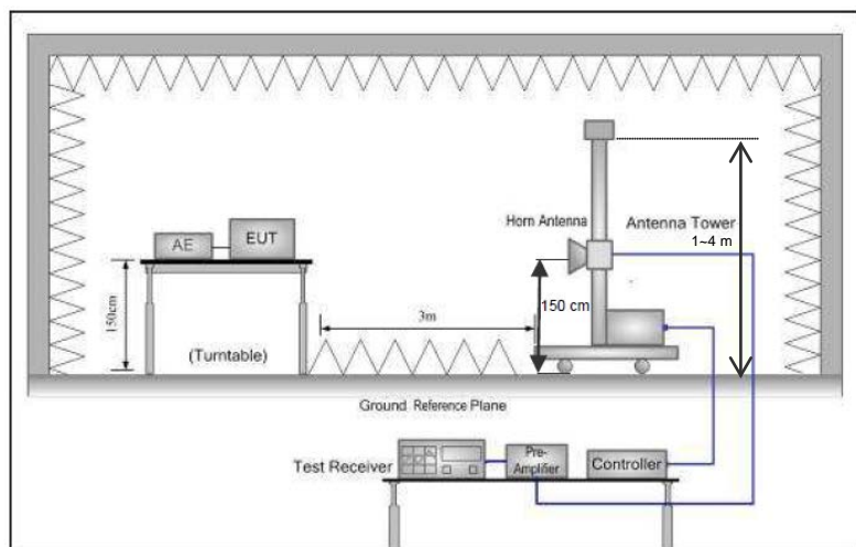
Above 1GHz
