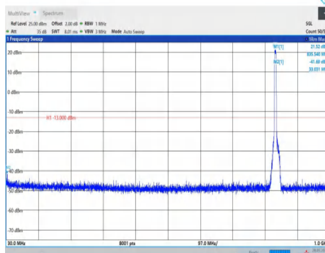
Band5-4182-30~1000MHz
