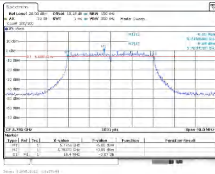
11A-CDD_Ant2_5785
