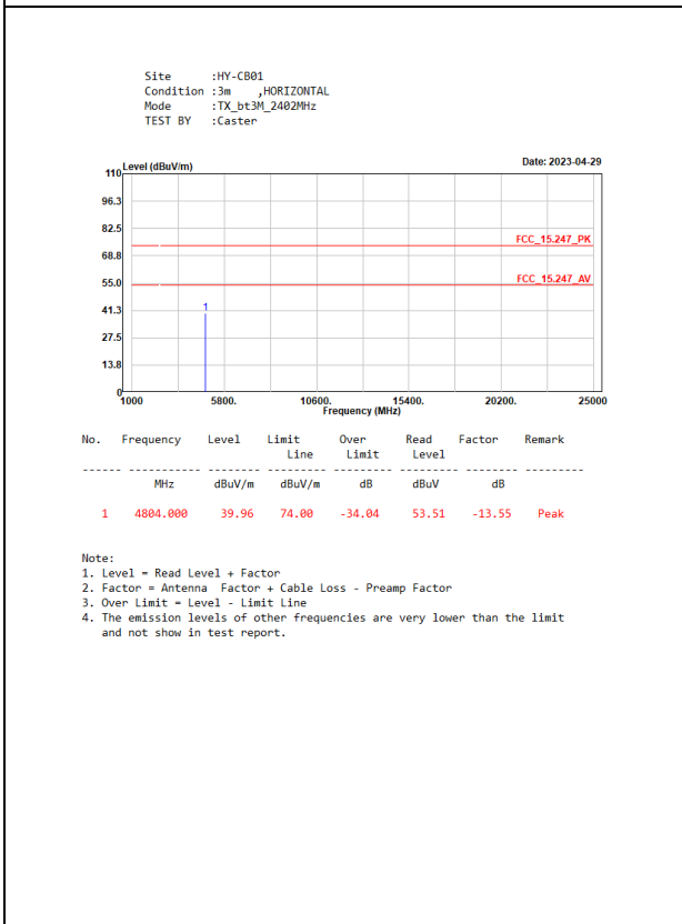
TX_bt3M_2402MHz_H_001
