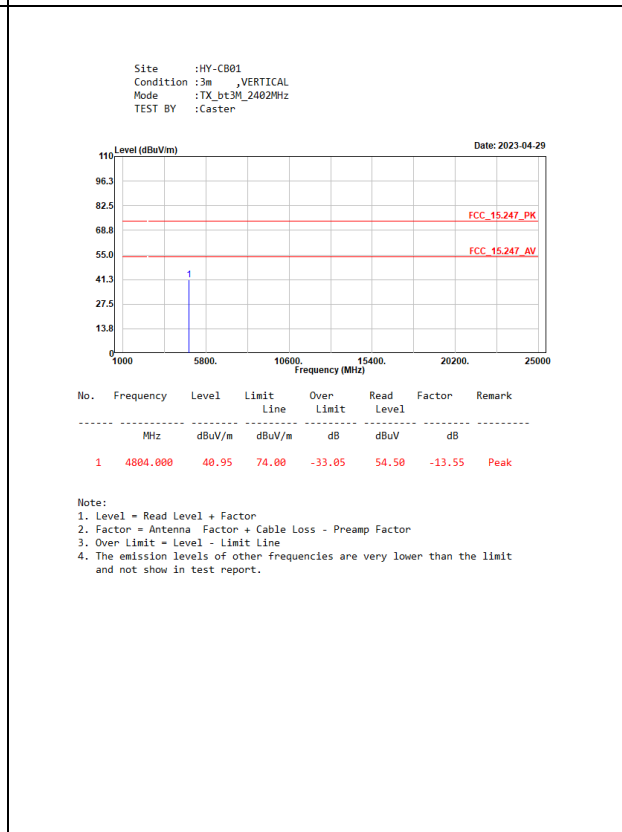
TX_bt3M_2402MHz_V_001
