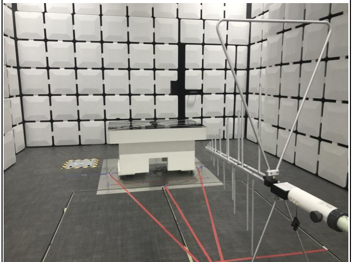
RADIATED BACK PHOTO (BELOW 1 GHz)
