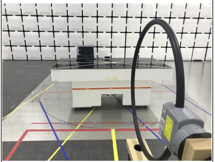
RADIATED BACK PHOTO (BELOW 30 GHz)
