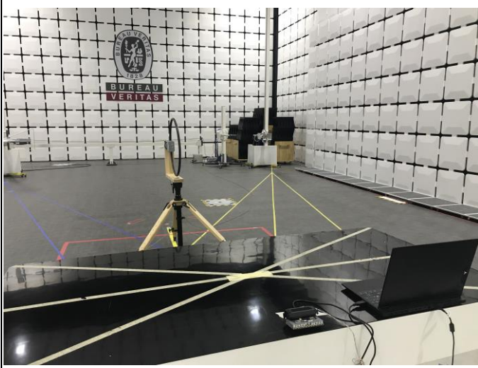
RADIATED FRONT PHOTO (BELOW 30 GHz)
