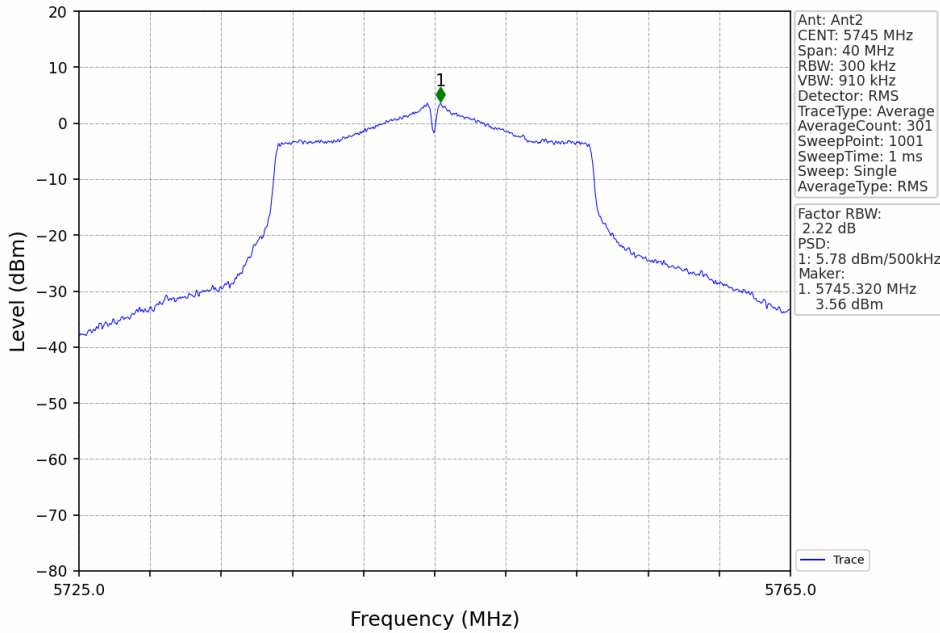
802.11ac(VHT20)_LCH_5745MHz_MIMO_NTNV
