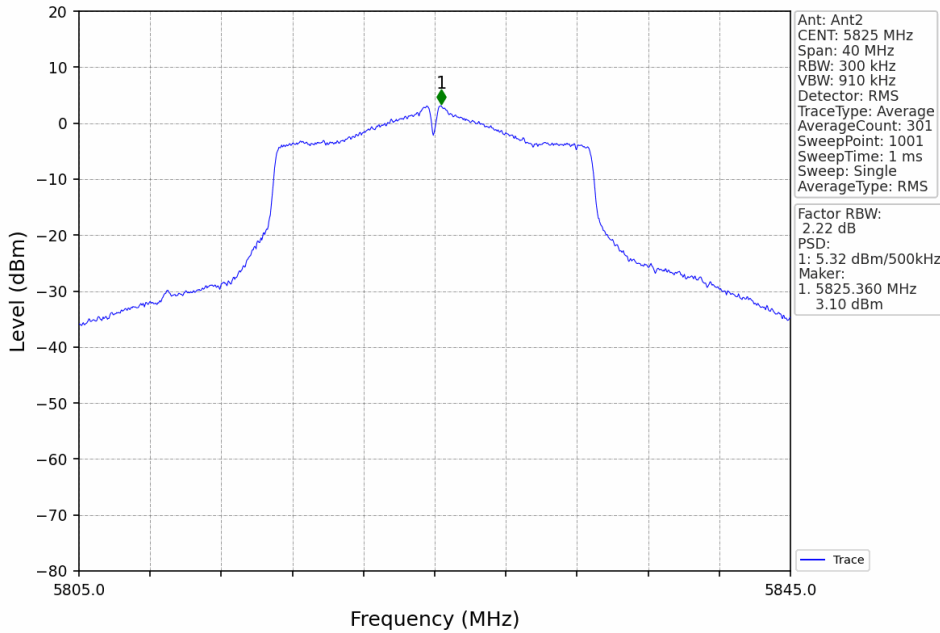
802.11ac(VHT20)_HCH_5825MHz_MIMO_NTNV
