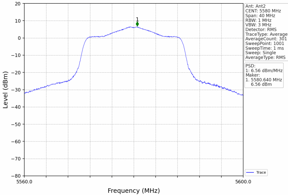
802.11ac(VHT20)_MCH_5580MHz_MIMO_NTNV
