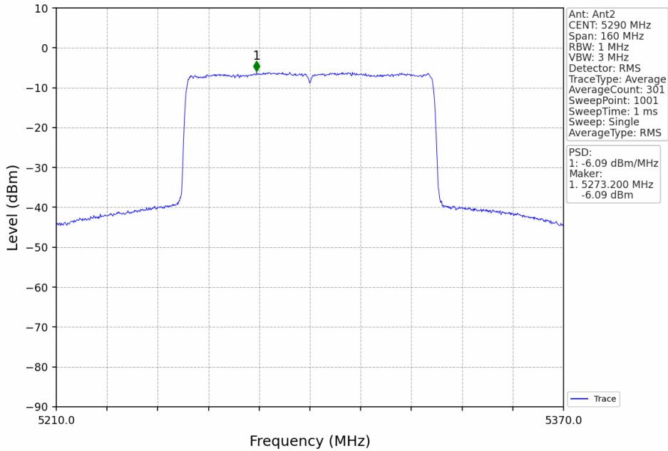
802.11ax(HEW80)_MCH_5290MHz_RU996_Left_MIMO_NTNV
