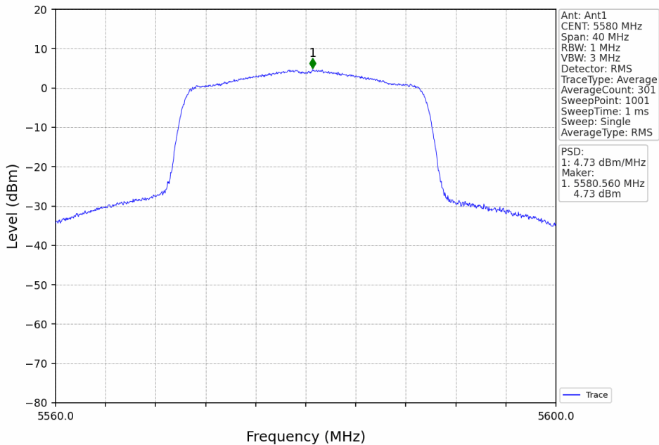
802.11ax(HEW20)_MCH_5580MHz_RU242_Left_Ant1_NTNV
