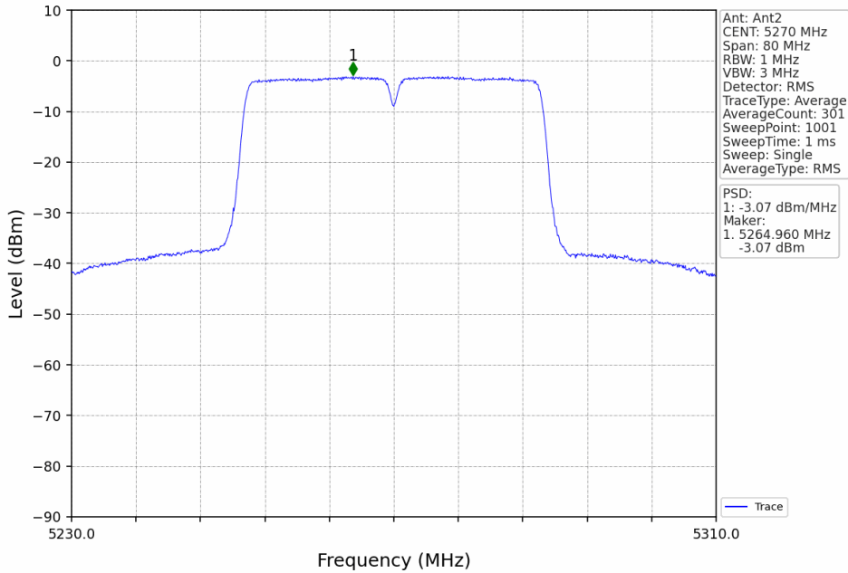
802.11ac(VHT40)_LCH_5270MHz_MIMO_NTNV
