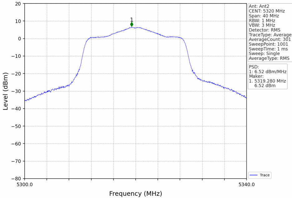
802.11ac(VHT20)_HCH_5320MHz_MIMO_NTNV
