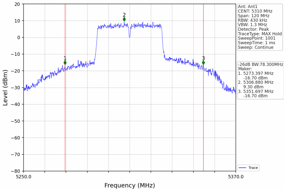
802.11ac(VHT40)_HCH_5310MHz_Ant1_NTNV
