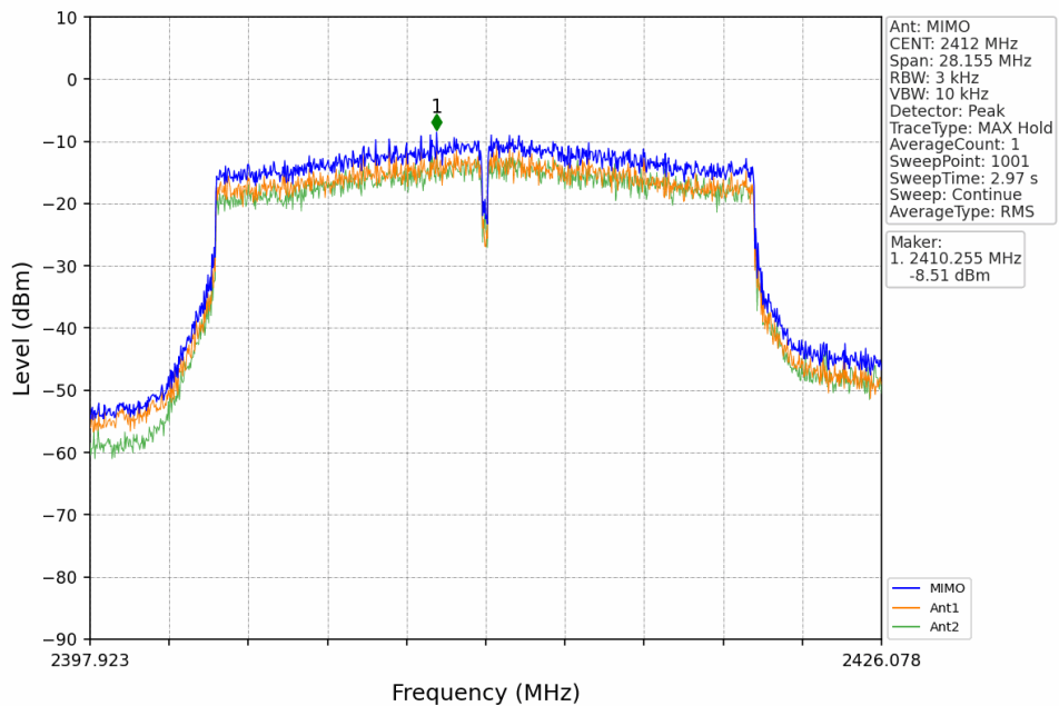
802.11ax(HEW20)_LCH_2412MHz_RU242_Left_MIMO_NTNV
