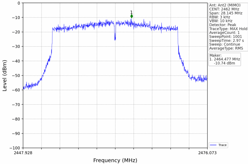
802.11ax(HEW20)_HCH_2462MHz_RU242_Left_MIMO_NTNV
