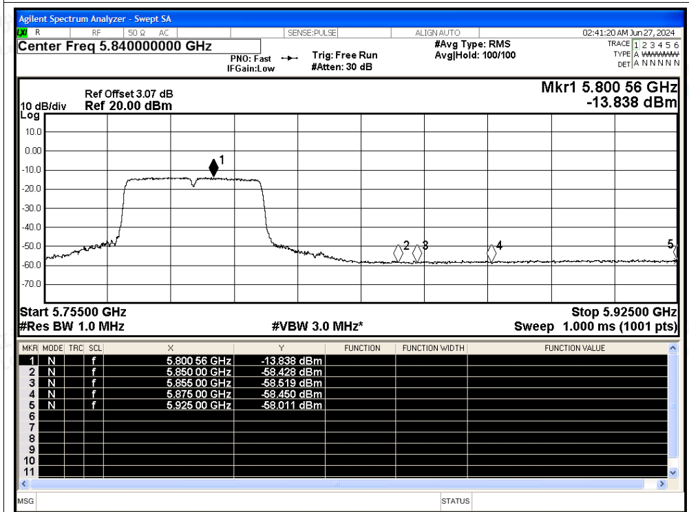
Restrict Band NVNT ac40 5795MHz Ant Average
