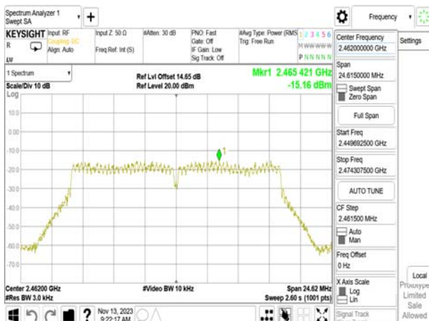
802.11g_20MHz_WLAN1_2462MHz
