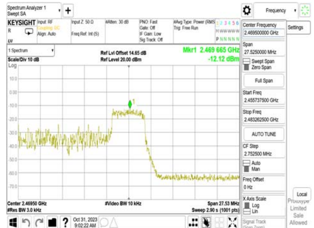
802.11ax_20MHz_WLAN2_2462MHz_RU106_54
