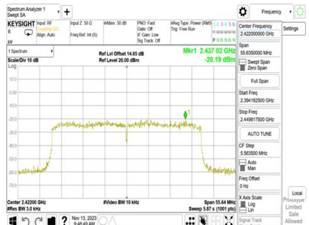
802.11ax_40MHz_WLAN2_2422MHz
