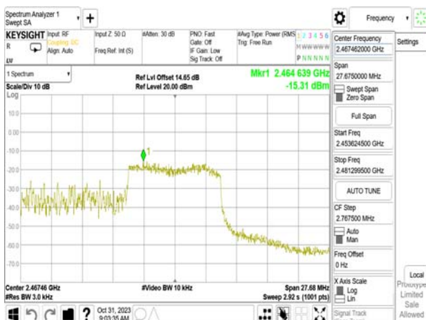
802.11ax_20MHz_WLAN1_2462MHz_RU106_54
