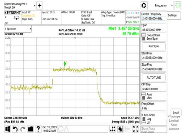
802.11ax_40MHz_WLAN2_2452MHz_RU242_62
