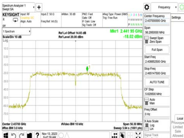
802.11ax_40MHz_WLAN1_2437MHz
