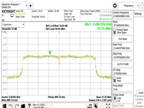
802.11ax_20MHz_WLAN2_2462MHz
