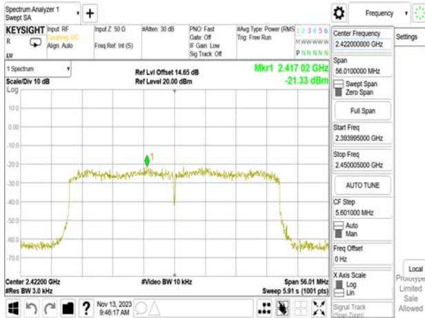
802.11ax_40MHz_WLAN1_2422MHz_RU242_61
