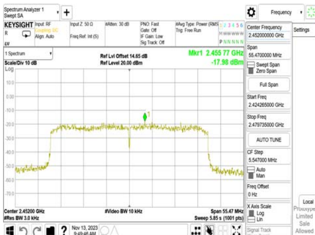
802.11ax_40MHz_WLAN2_2452MHz
