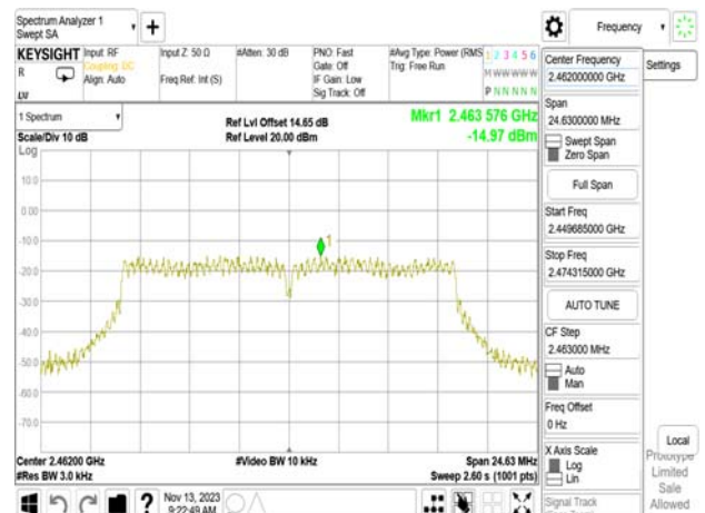
802.11g_20MHz_WLAN2_2462MHz
