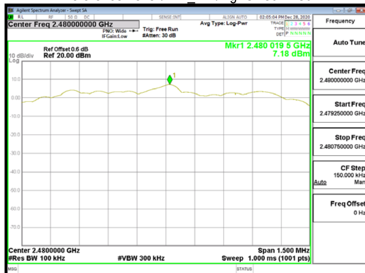
Reference Level\BLE_2M\HighCH39-2480
