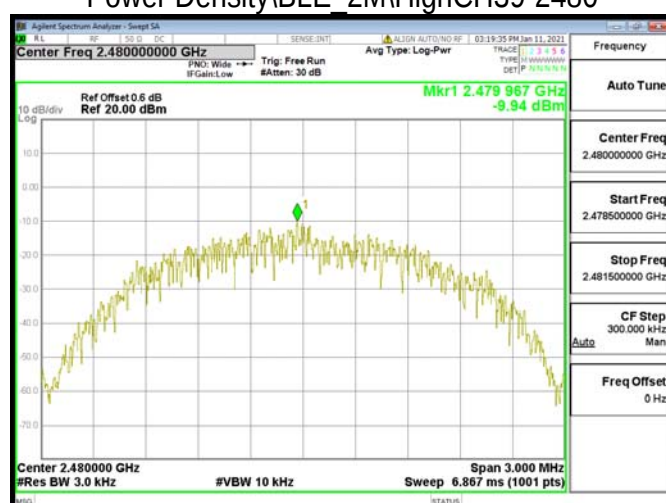
Power Density\BLE 2M\HighCH39-2480
