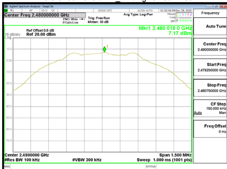
Reference Level\BLE_1M\HighCH39-2480
