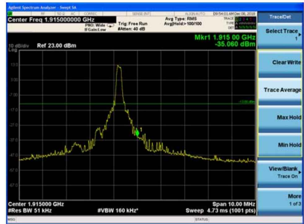
LTE Band 25 10MHz QPSK 100%RB CH-High
