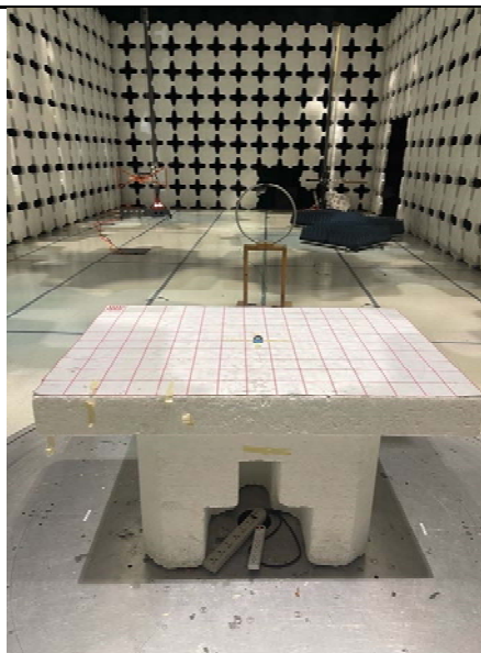
Radiated Emission Test below 30 MHz Rear View
