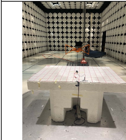
Radiated Emission Test below 1GHz Front View
