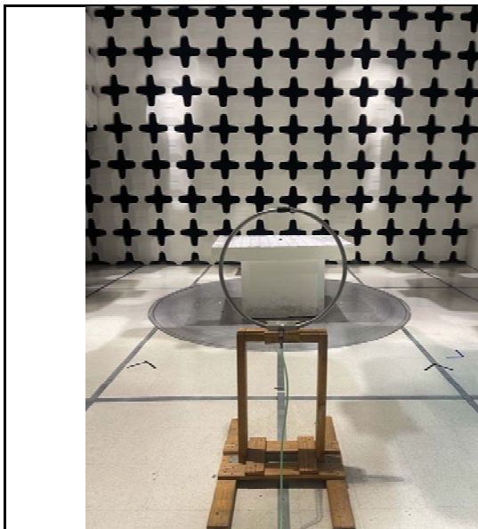
Radiated Emission Test below 30MHz Front View
