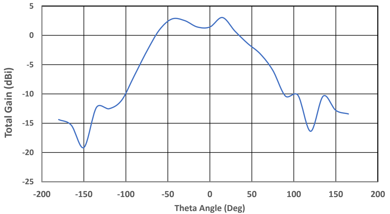
EDV VAS Rectangular Ground Plane PT0039230 2422 MHz Phi=0 degrees
