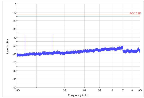
LTE Band 26 5MHz CH-Middle 1.5GHz~9GHz
