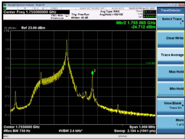
NB-IOT Band 4 QPSK 15kHz 1@11CH-High
