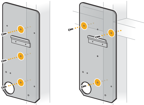
Vertical Stud Installation
