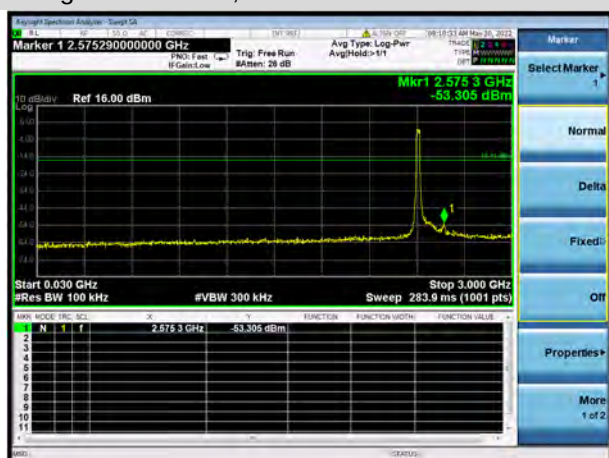
802.11g 1 CHANNEL, SPURIOUS 30 MHz ~ 3 GHz
