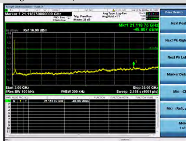
802.11g 1 CHANNEL, SPURIOUS 2 GHz ~ 25 GHz
