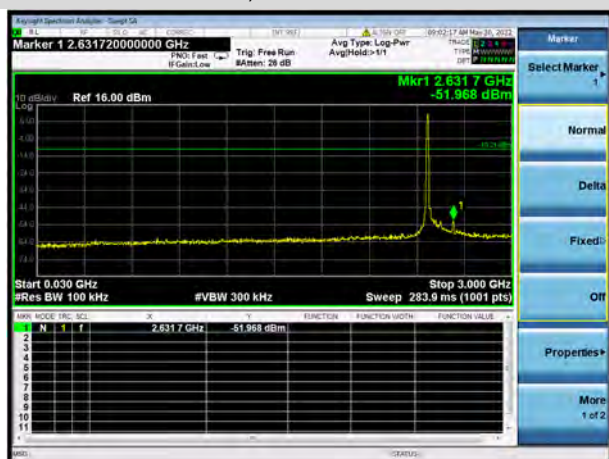
802.11b 13 CHANNEL, SPURIOUS 30 MHz ~ 3 GHz
