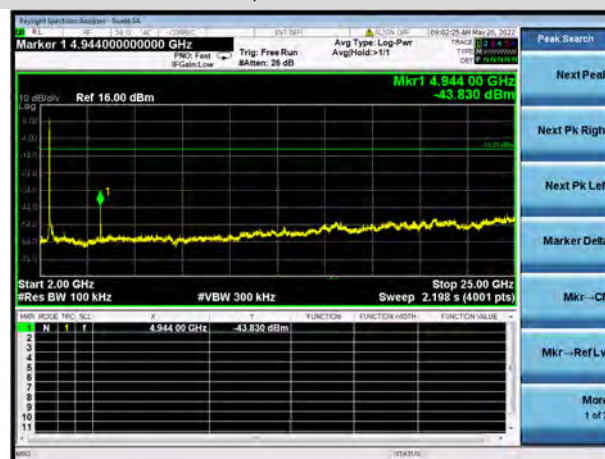
802.11b 13 CHANNEL, SPURIOUS 2 GHz ~ 25 GHz
