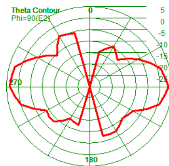
Efficiency:73.1%
