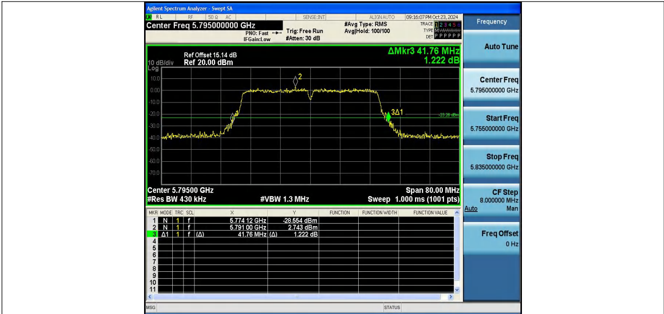
11AC40SISO-Ant2-5795
