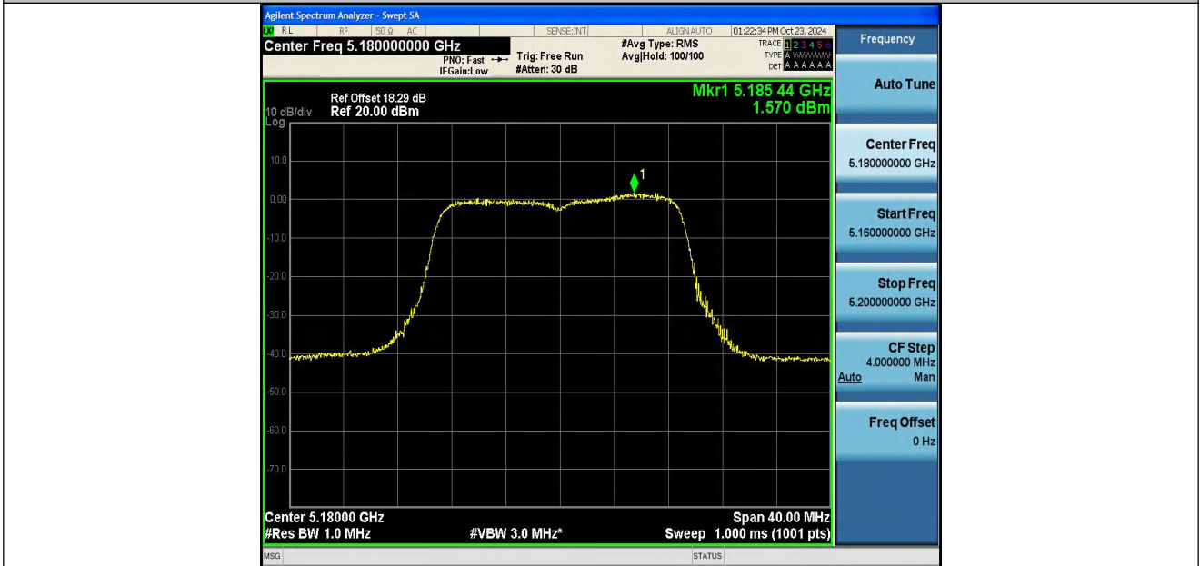
11N20SISO-Ant2-5180-PASS
