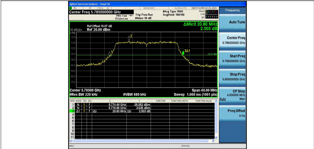
11AC20SISO-Ant2-5785
