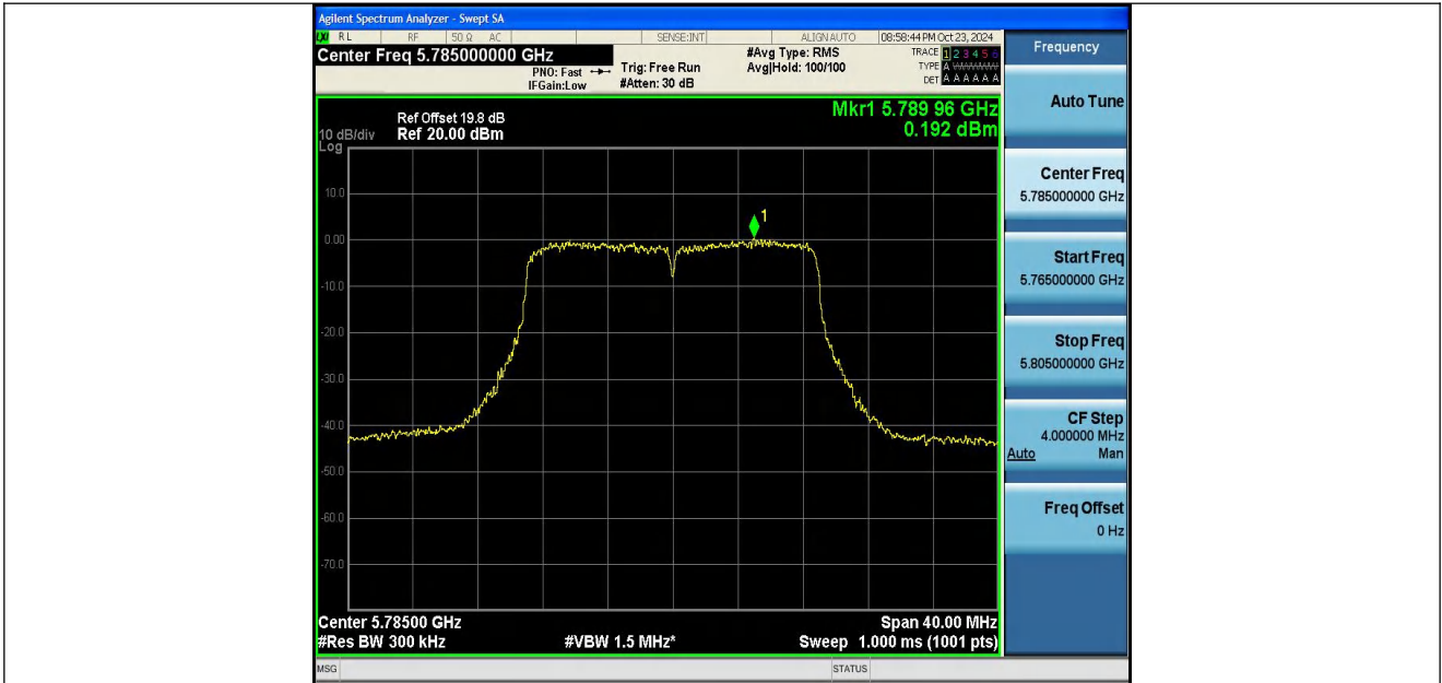
11AC20SISO-Ant2-5785-PASS
