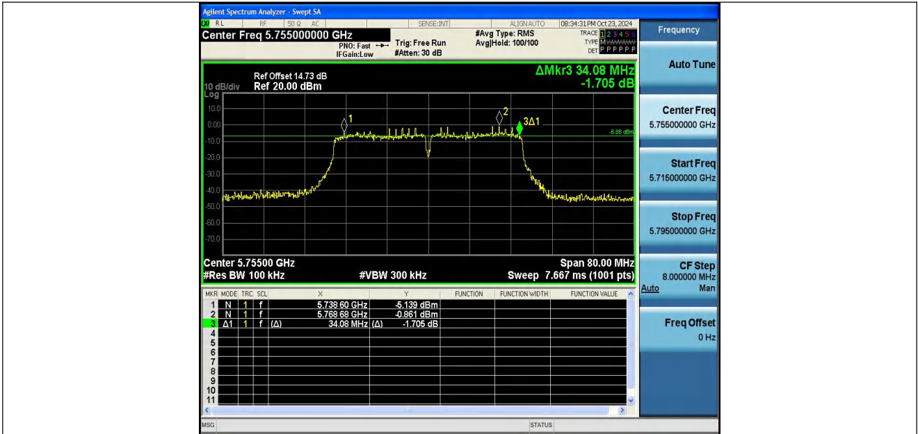
11N40SISO-Ant2-5755-PASS
