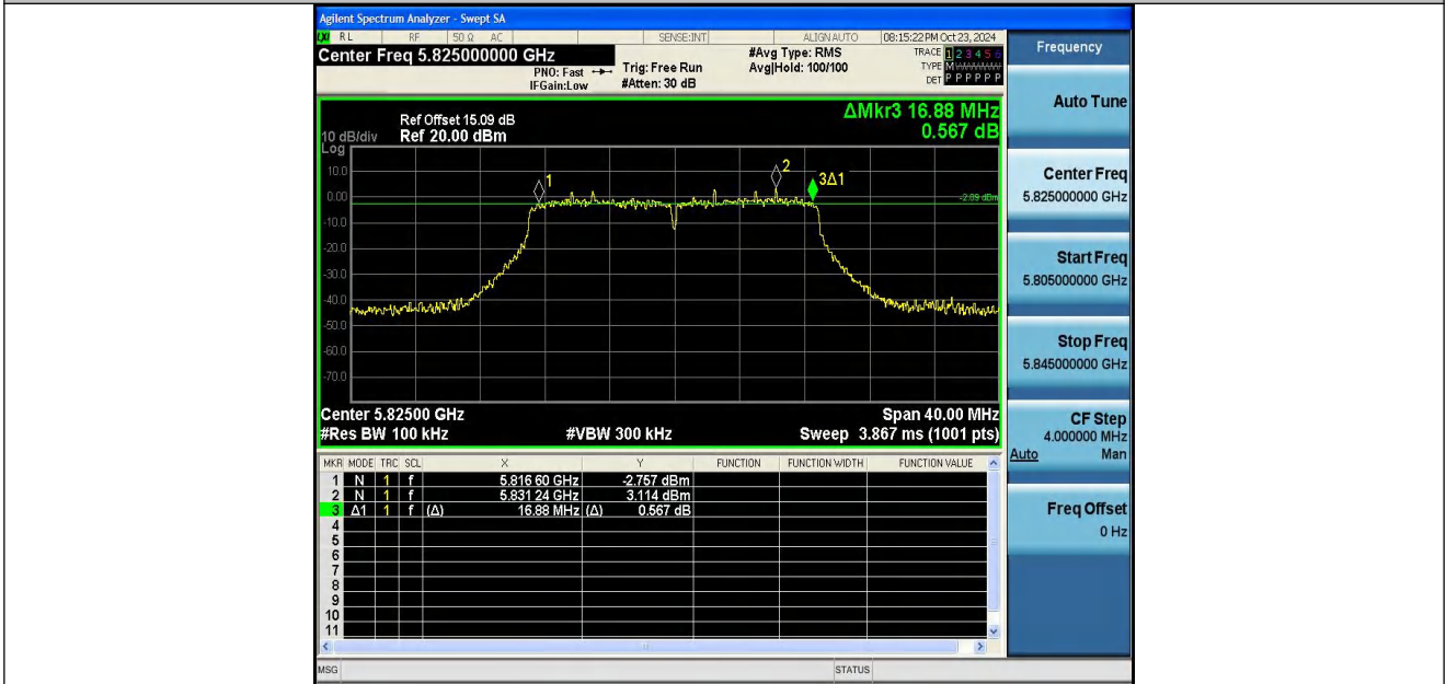
11N20SISO-Ant2-5825-PASS
