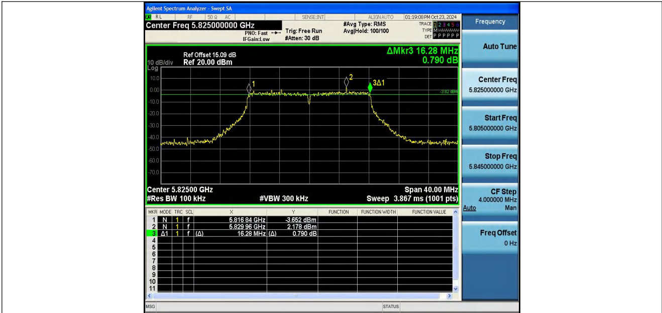
11A-Ant2-5825-PASS
