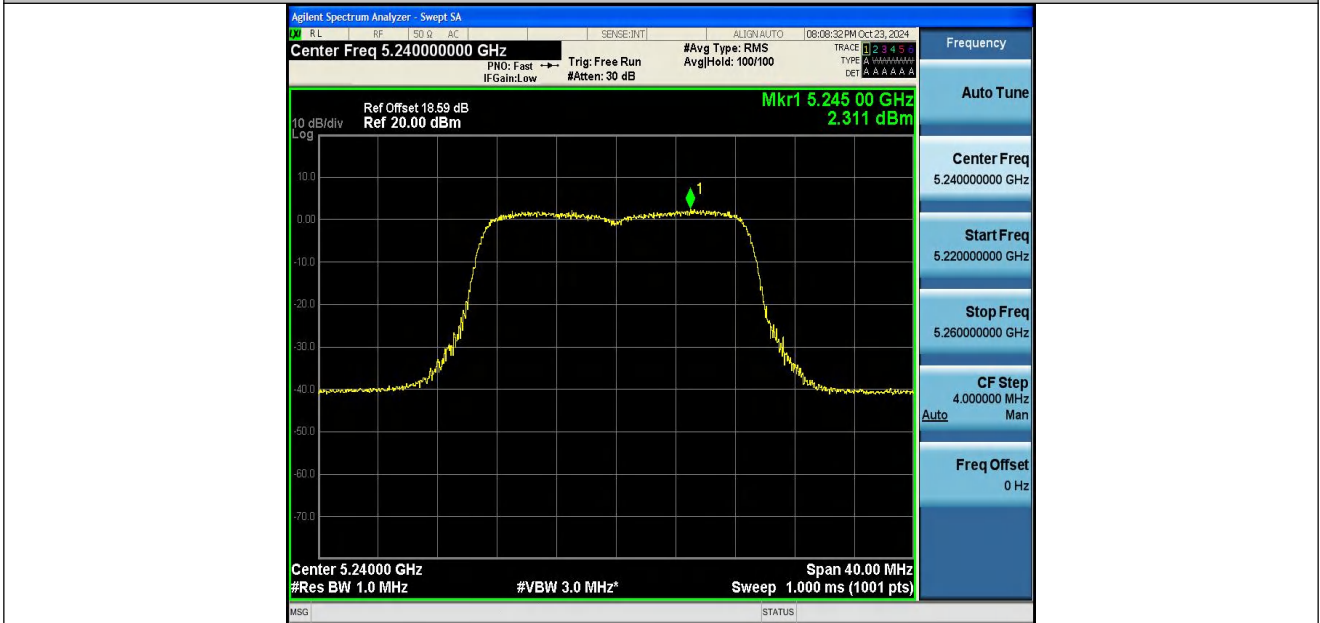
11N20SISO-Ant2-5240-PASS
