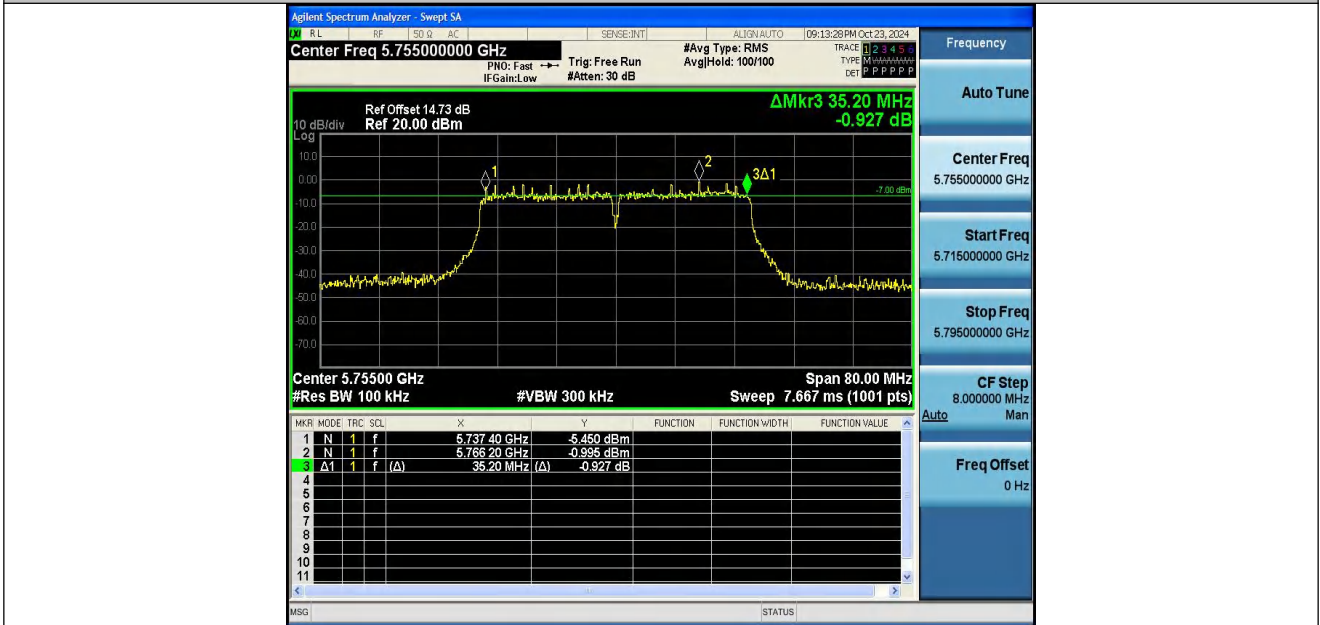
11AC40SISO-Ant2-5755-PASS
