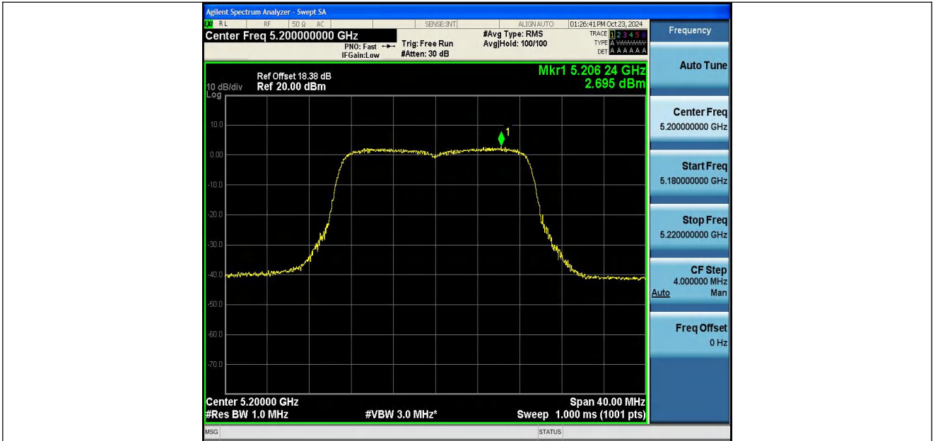
11N20SISO-Ant2-5200-PASS
