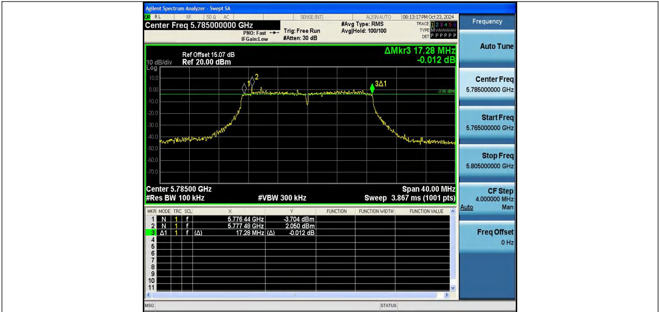
11N20SISO-Ant2-5785-PASS
