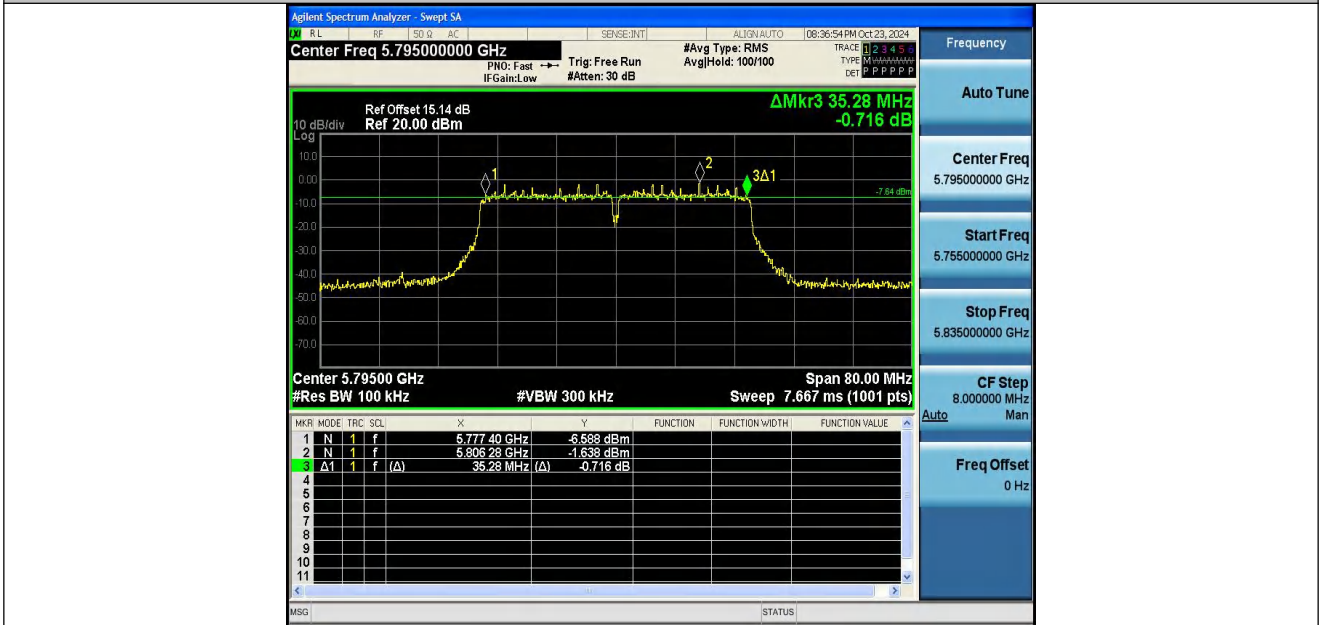
11N40SISO-Ant2-5795-PASS
