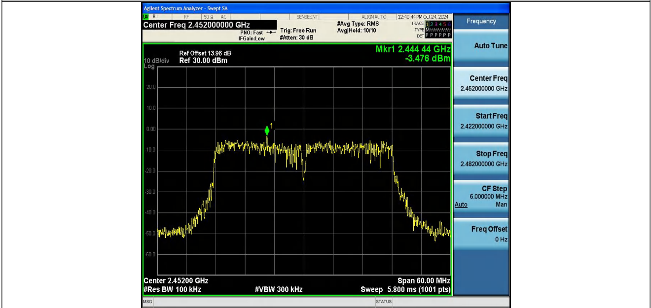
11N40SISO-Ant1-2452-0~Reference-PASS
