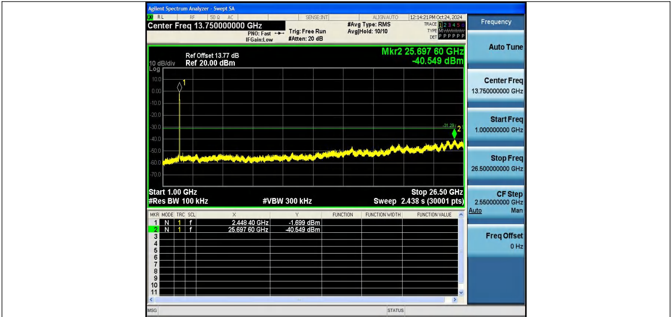
11N40SISO-Ant1-2437-1000~26500-PASS
