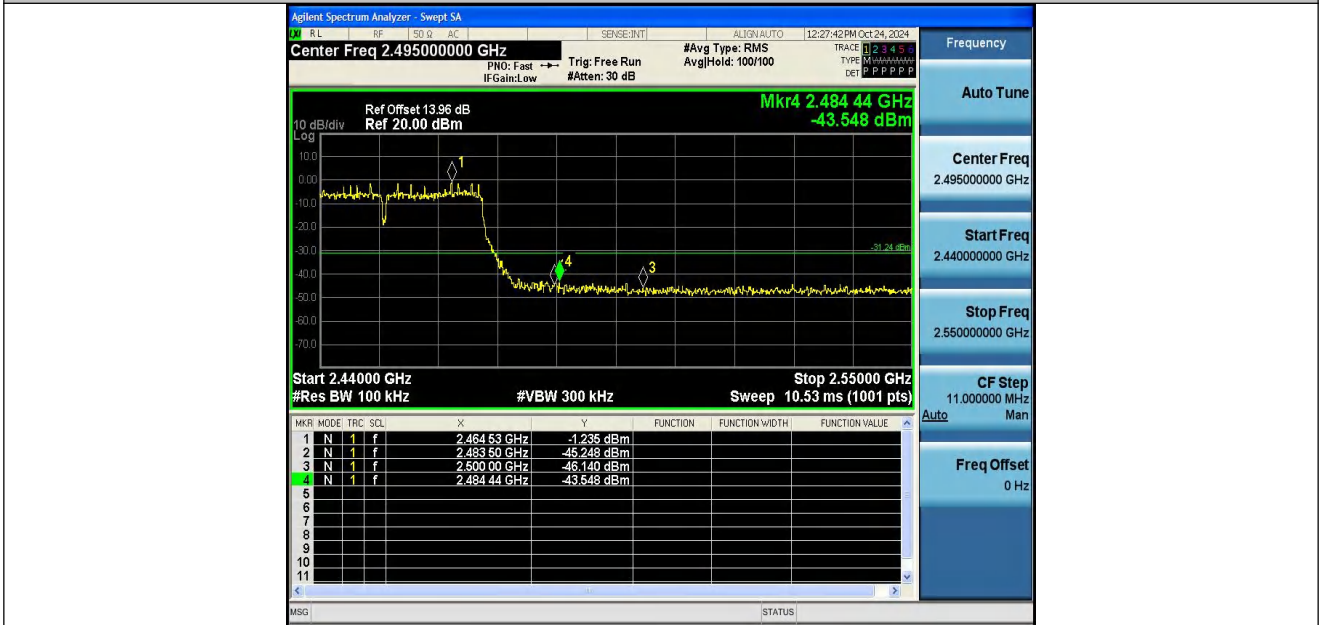
11N40SISO-Ant1-2452-PASS
