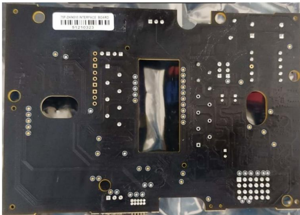
HyperStat Interface Daikin P1P2 Base PCB back view
