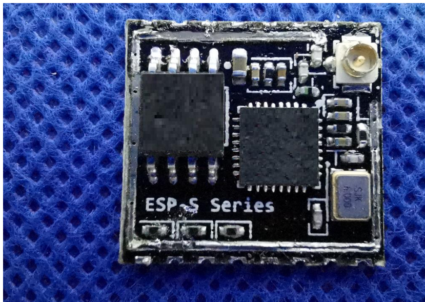
Photo 9(wifi module)
