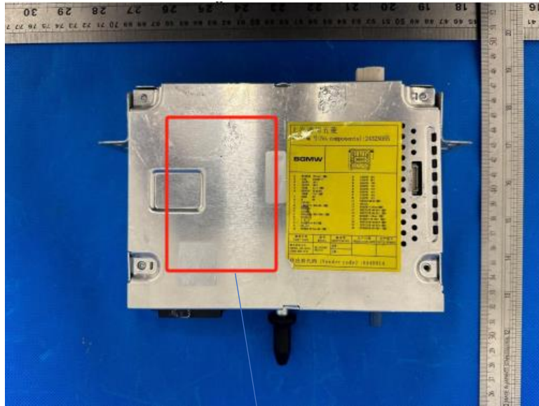
Label location
