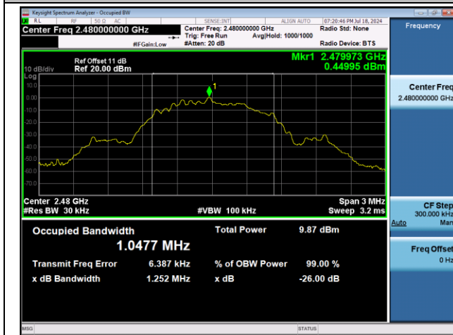
BLE_1M-Ant1-2480
