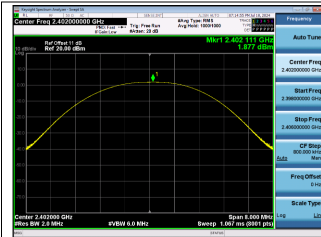
BLE_1M-Ant1-2402-PASS
