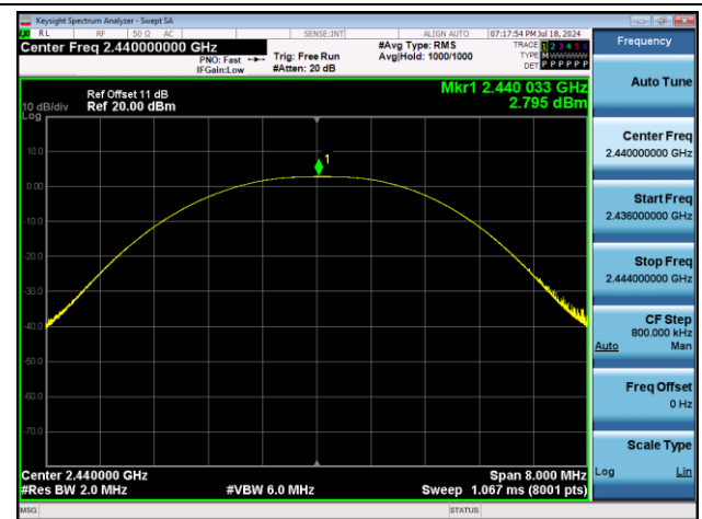
BLE_1M-Ant1-2440-PASS
