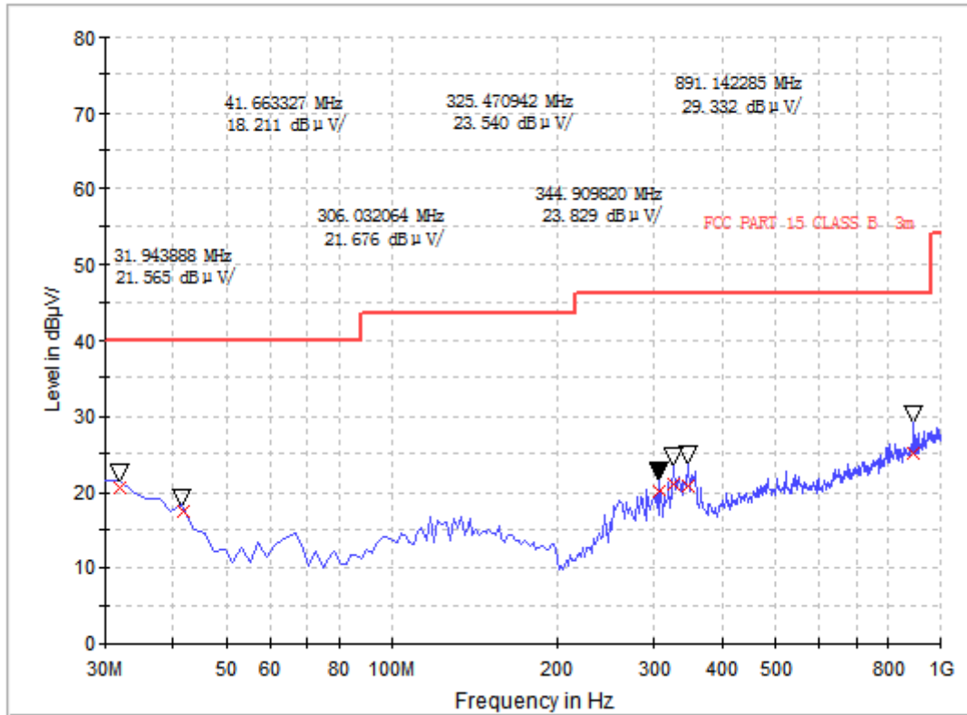
EMI Sweep-3M(30-1G)
