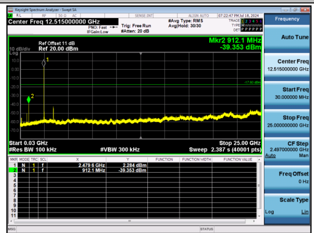
BLE_1M-Ant1-2480-30~25000-PASS
