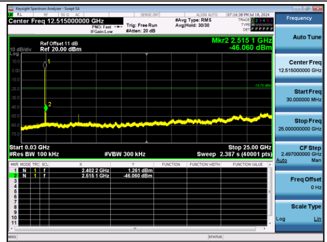
BLE_1M-Ant1-2402-30~25000-PASS
