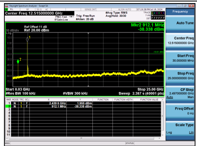
BLE_1M-Ant1-2440-30~25000-PASS
