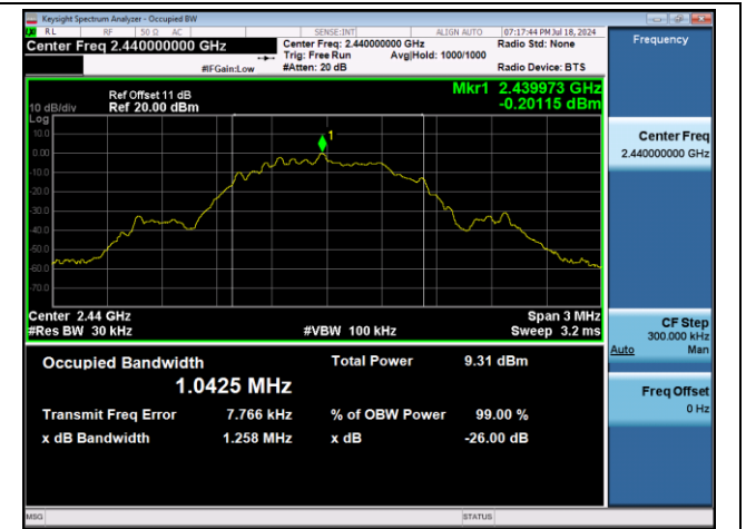
BLE_1M-Ant1-2440
