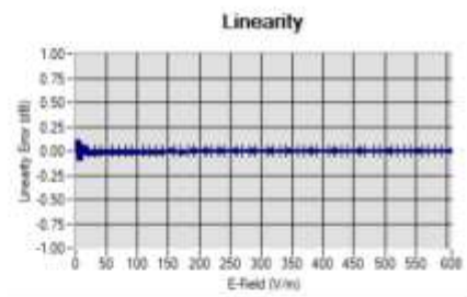
Linearity +/-1.87% (+/-0.08dB)
