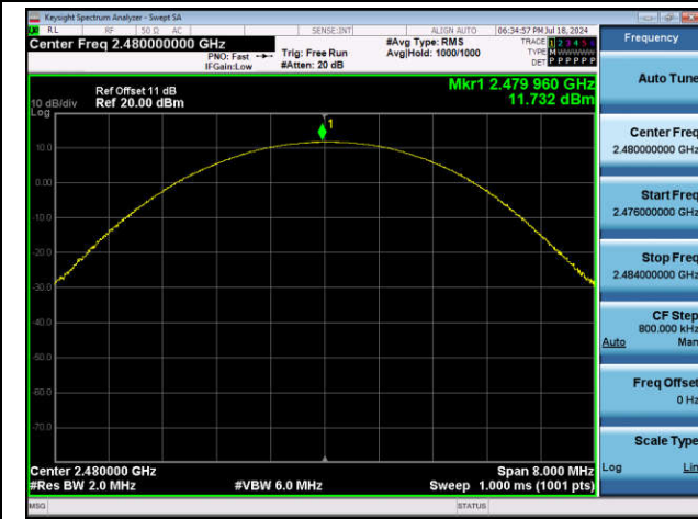
3DH5-Ant1-2480-PASS
