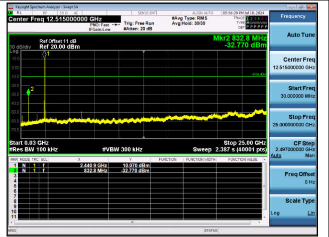
DH5-Ant1-2441-30~25000-PASS
