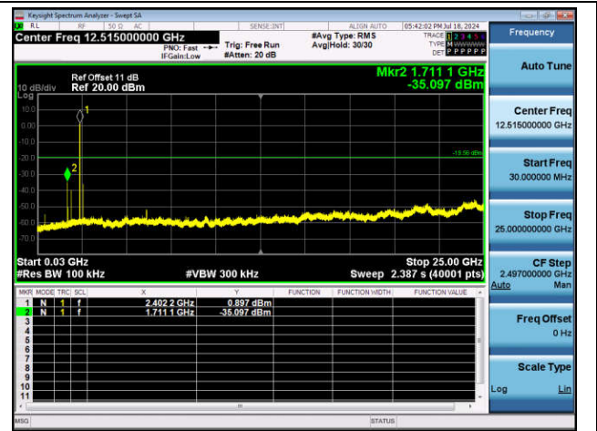
DH5-Ant1-2402-30~25000-PASS
