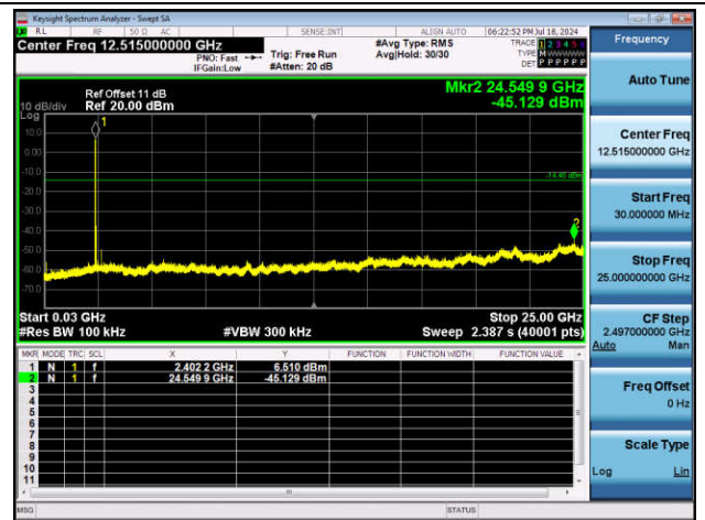
3DH5-Ant1-2402-30~25000-PASS
