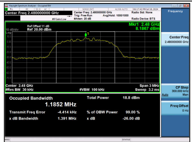
2DH5-Ant1-2480
