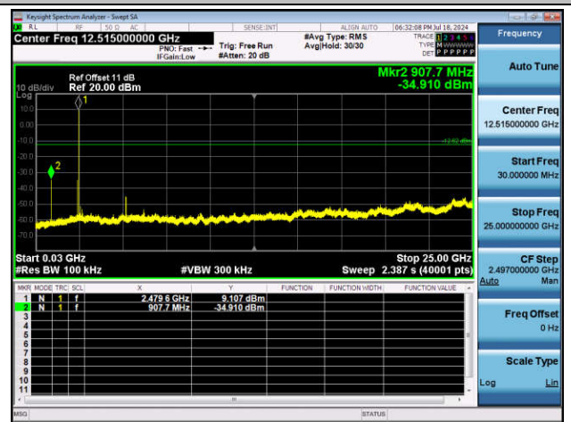
3DH5-Ant1-2480-30~25000-PASS
