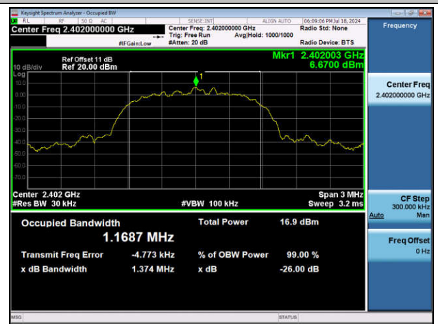
2DH5-Ant1-2402
