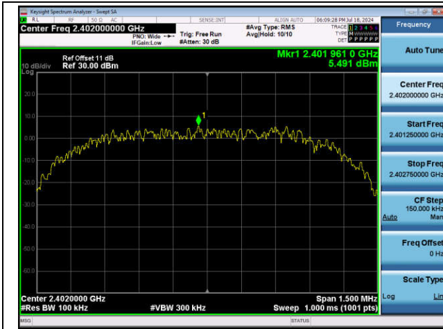
2DH5-Ant1-2402-0~Reference-PASS
