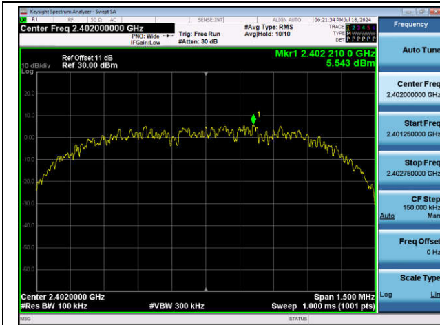
3DH5-Ant1-2402-0~Reference-PASS
