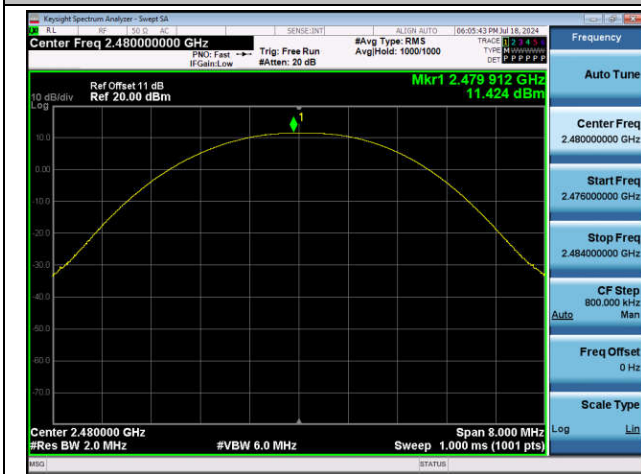
DH5-Ant1-2480-PASS
