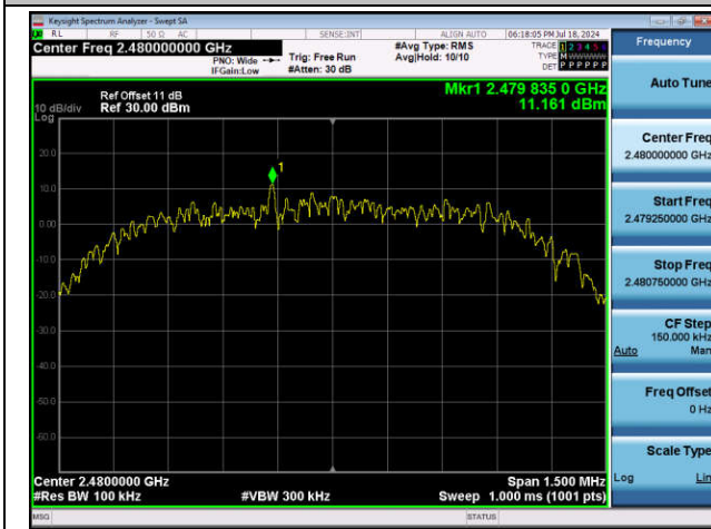
2DH5-Ant1-2480-0~Reference-PASS
