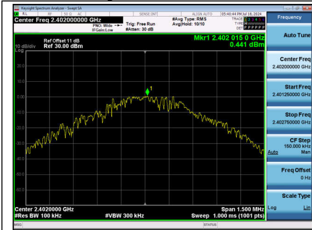
DH5-Ant1-2402-0~Reference-PASS
