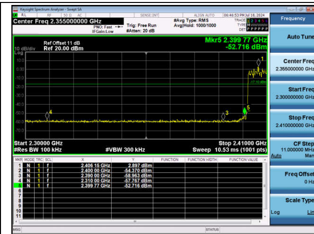
2DH5-Ant1-Hop_2402-PASS
