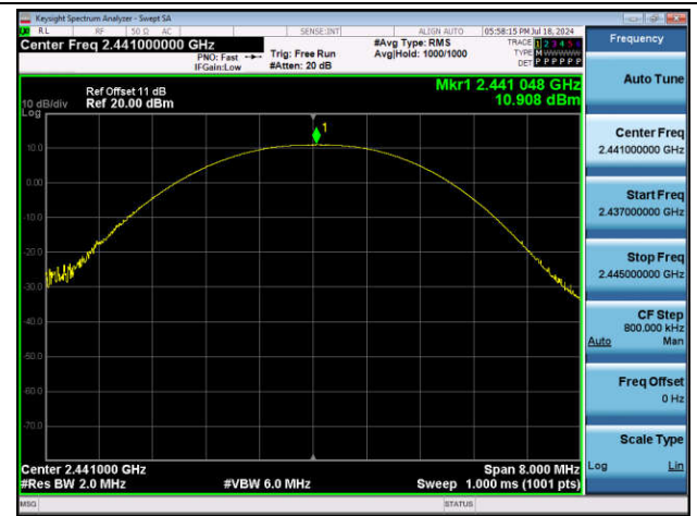
DH5-Ant1-2441-PASS
