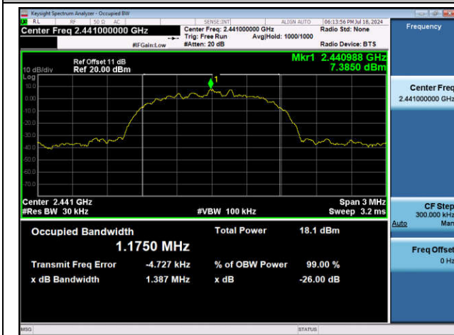
2DH5-Ant1-2441
