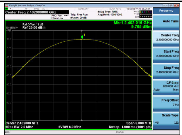
2DH5-Ant1-2402-PASS
