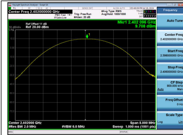
DH5-Ant1-2402-PASS
