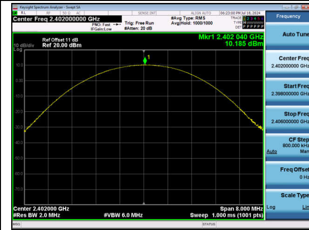
3DH5-Ant1-2402-PASS
