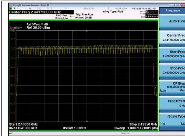
DH5-Ant1-Hop-PASS
