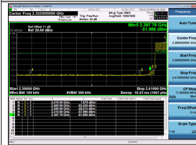
DH5-Ant1-Hop_2402-PASS
