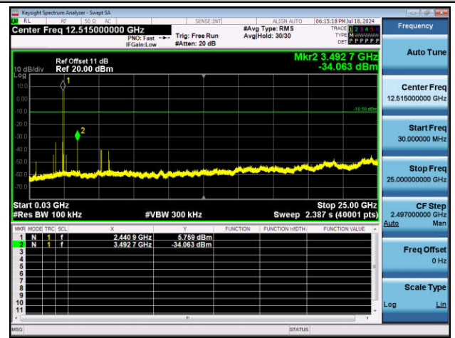
2DH5-Ant1-2441-30~25000-PASS
