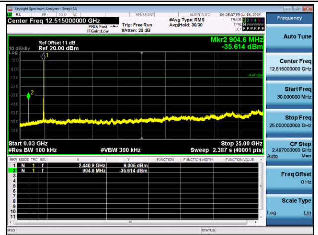
3DH5-Ant1-2441-30~25000-PASS
