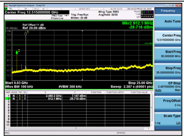
2DH5-Ant1-2480-30~25000-PASS
