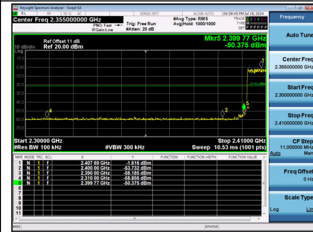
3DH5-Ant1-Hop_2402-PASS
