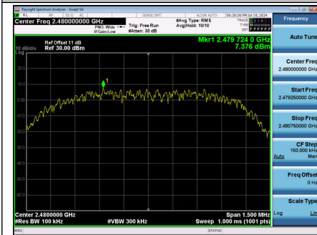
3DH5-Ant1-2480-0~Reference-PASS
