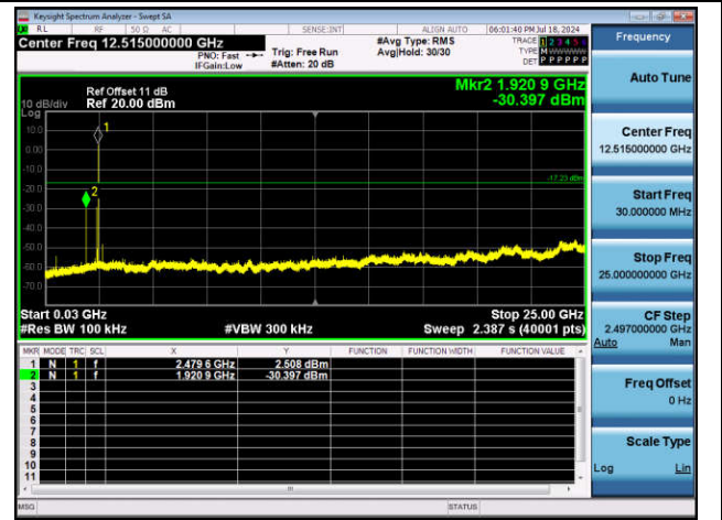
DH5-Ant1-2480-30~25000-PASS
