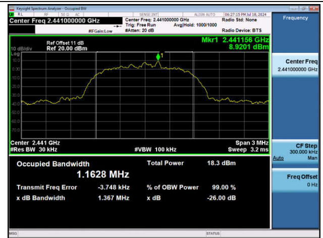
3DH5-Ant1-2441
