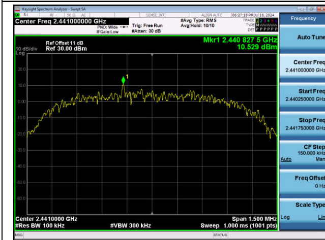
3DH5-Ant1-2441-0~Reference-PASS
