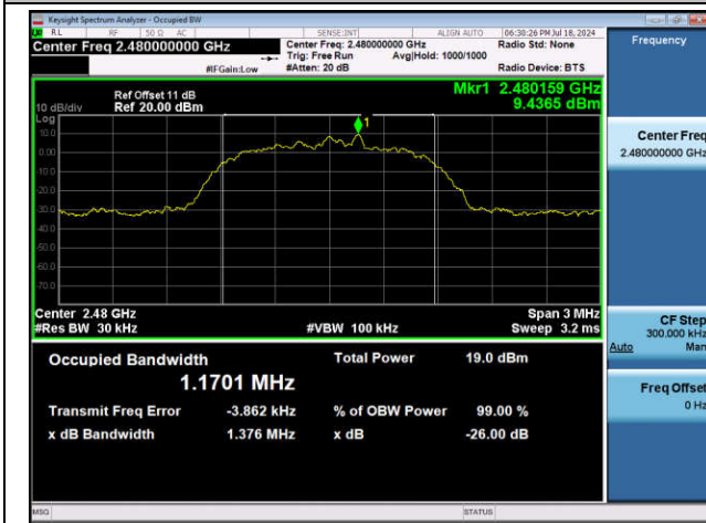
3DH5-Ant1-2480
