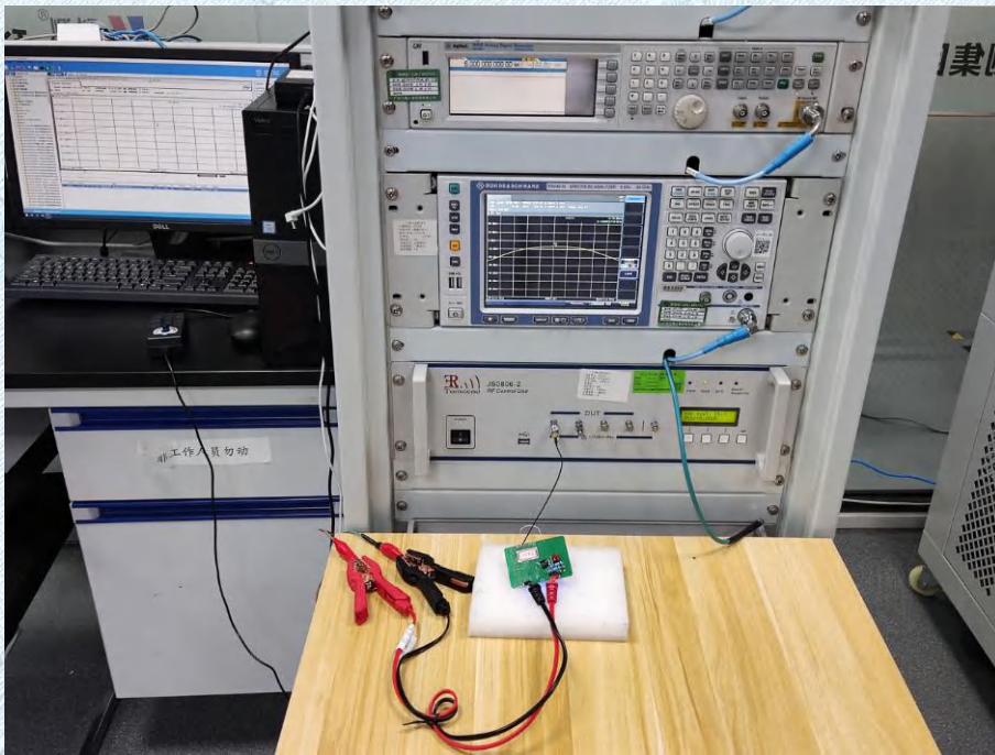
RF Conducted
