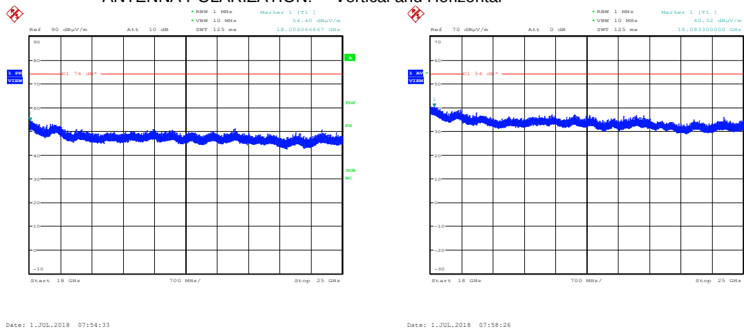
Plot 7.1.29 Radiated emission measurements from 18.0 to 25 GHz, mid frequency
