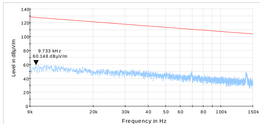
Plot 7.1.5 Radiated emission measurements from 9 to 150 kHz, mid frequency
