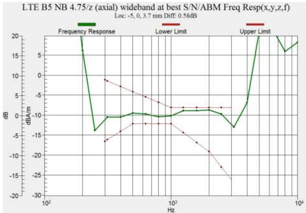
Figure B.11 Frequency Response of LTE Band 5
