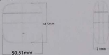
Charging box
