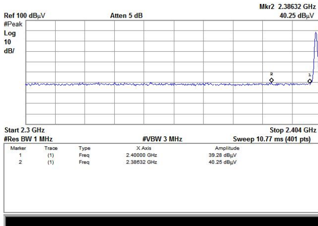
\pi/4 -DQPSK: Band Edge-Low Channel
