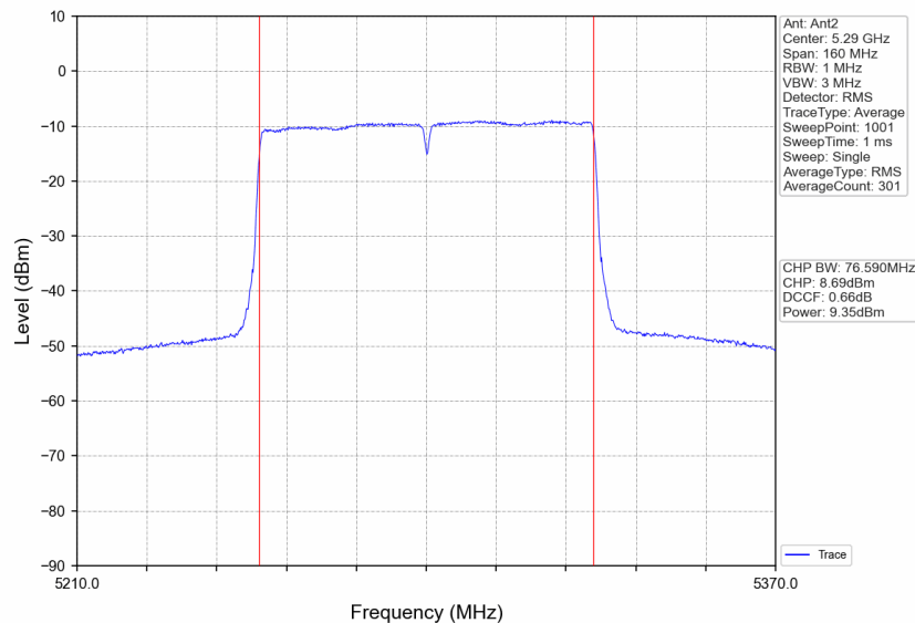
802.11ac(VHT80)_MCH_5290MHz_Ant2_NTNV
