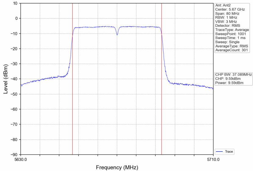
802.11ac(VHT40)_HCH_5670MHz_Ant2_NTNV
