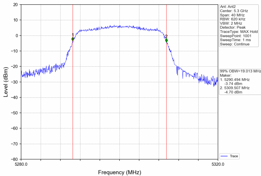
802.11ac(VHT20)_MCH_5300MHz_Ant2_NTNV
