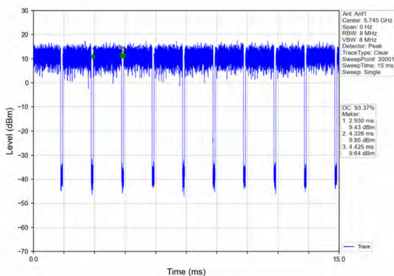
802.11a_LCH_5745MHz_Ant1_NTNV
