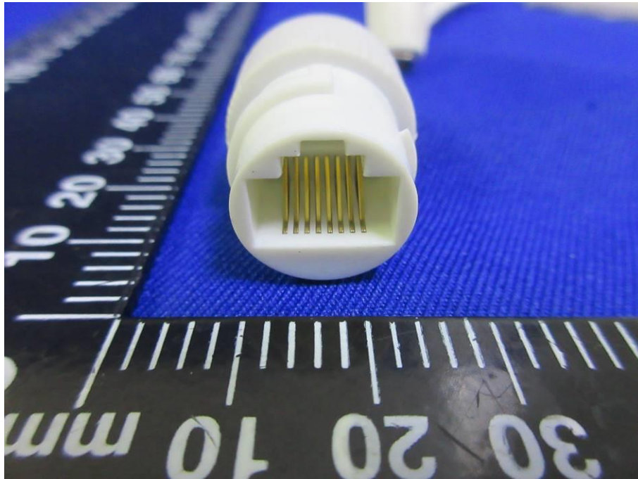
RJ45 Port
