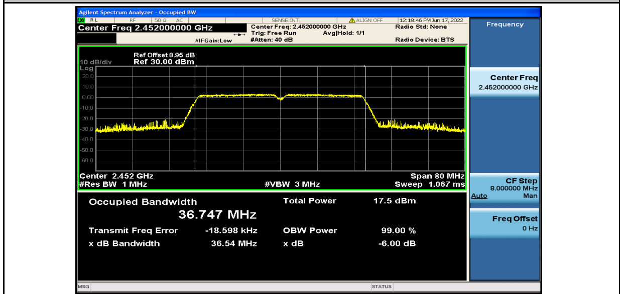
Occupied Bandwidth_11N40ISO_2452
