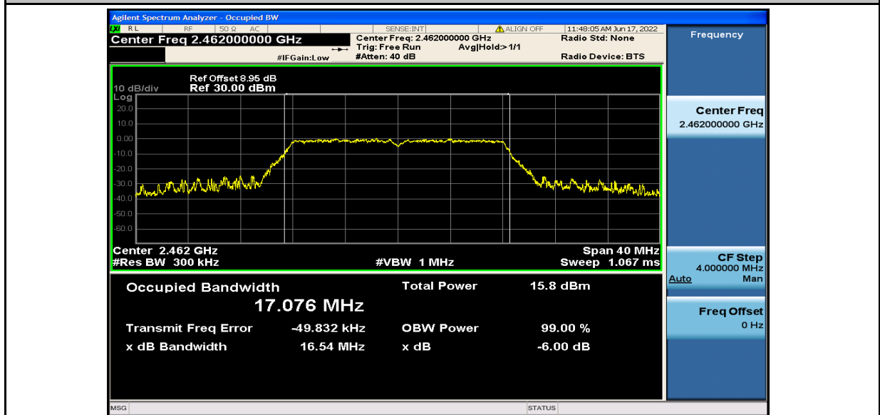
Occupied Bandwidth_11N20SISO_2412
