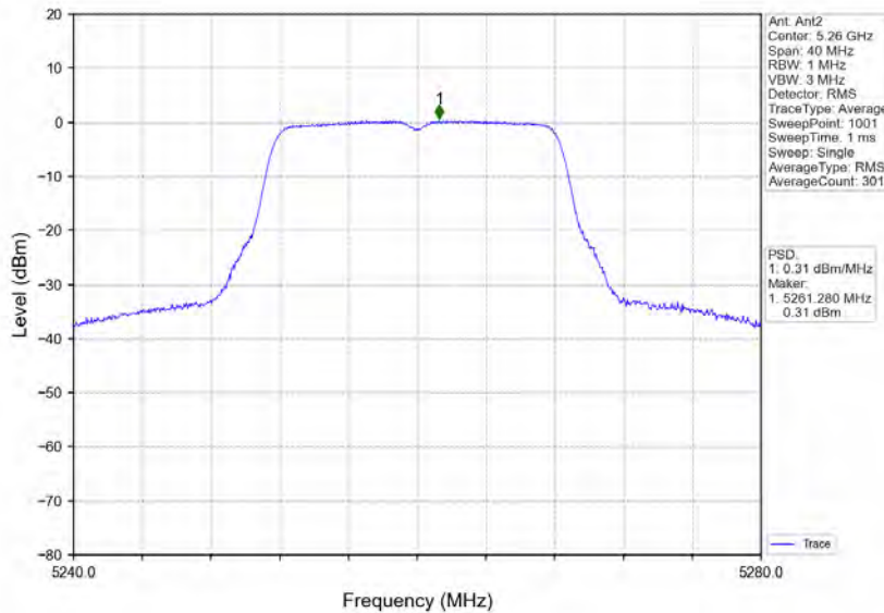
802.11a_LCH_5260MHz_Ant2_NTNV
