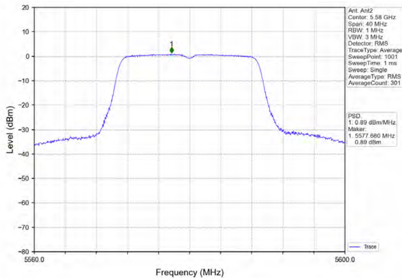
802.11n(HT20)_MCH_5580MHz_Ant2_NTNV
