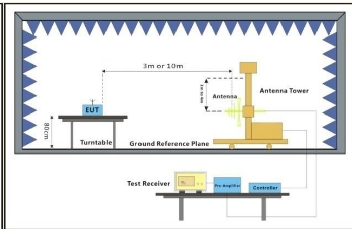
30MHz-1GHz
