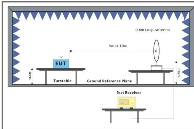
Below 30MHz
