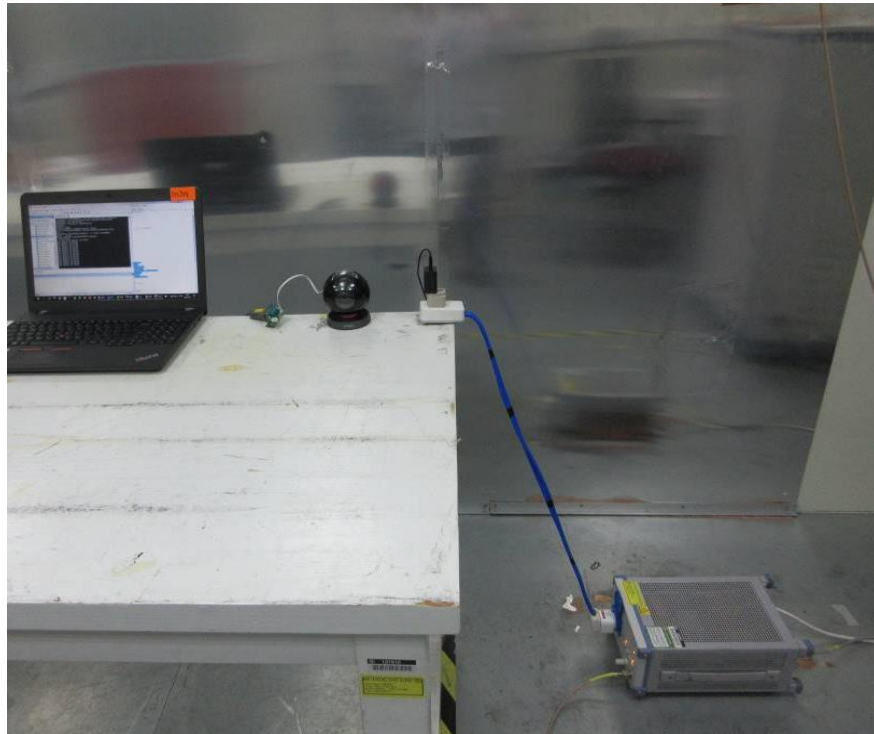
POWERLINE CONDUCTED EMISSIONS MEASUREMENT SETUP
