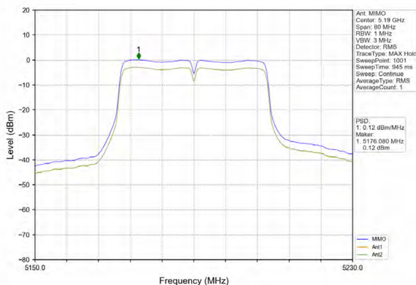
802.11n(HT40)_LCH_5190MHz_MIMO_NTNV
