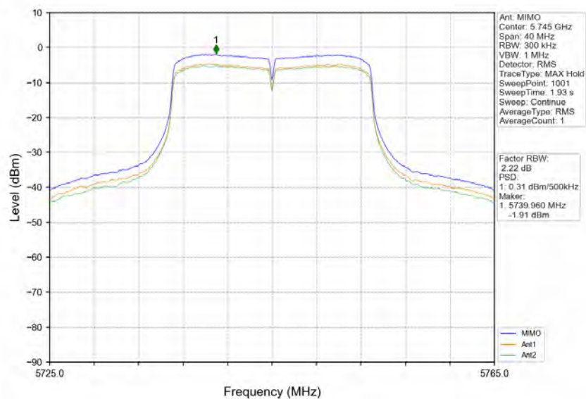
802.11ac(VHT20)_LCH_5745MHz_MIMO_NTNV
