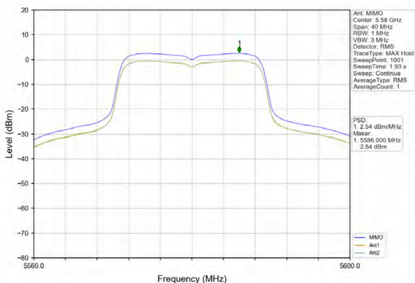
802.11ac(VHT20)_MCH_5580MHz_MIMO_NTNV
