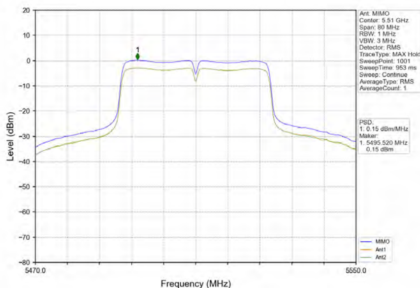
802.11ac(VHT40)_LCH_5510MHz_MIMO_NTNV
