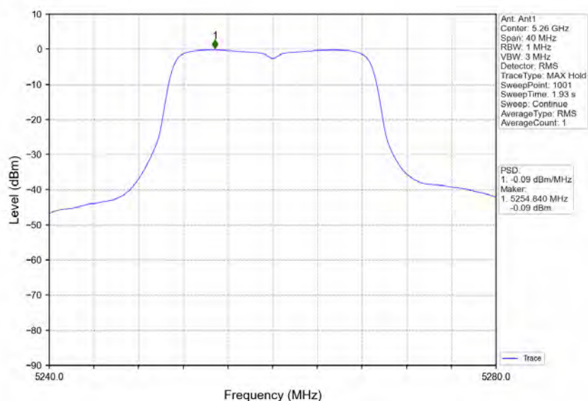
802.11ac(VHT20)_LCH_5260MHz_Ant1_NTNV
