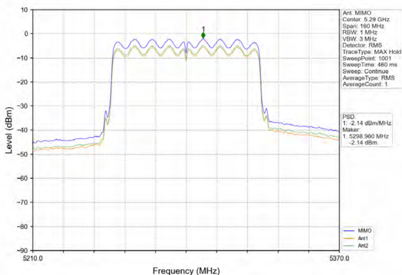
802.11ac(VHT80)_MCH_5290MHz_MIMO_NTNV
