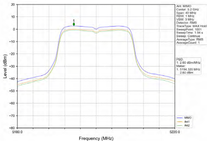
802.11ac(VHT20)_MCH_5200MHz_MIMO_NTNV
