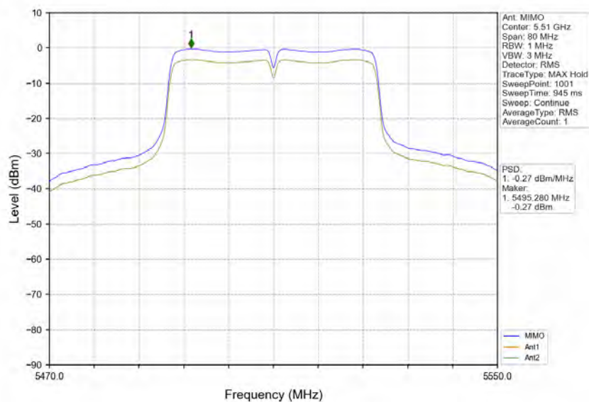
802.11n(HT40)_LCH_5510MHz_MIMO_NTNV
