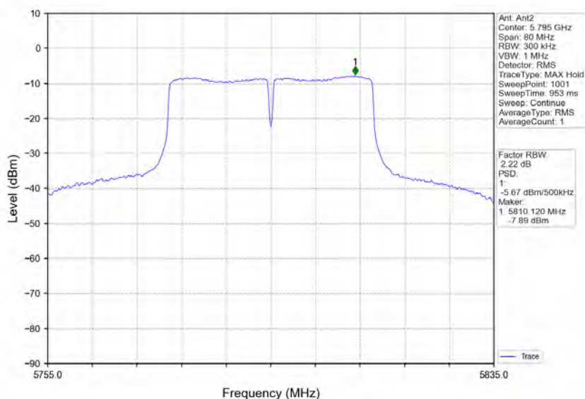
802.11ac(VHT40)_HCH_5795MHz_MIMO_NTNV
