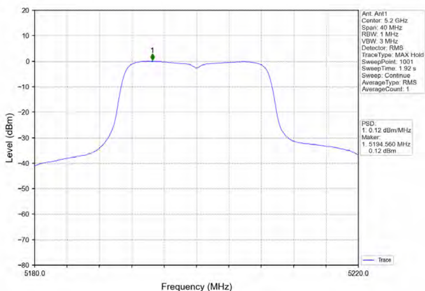
802.11n(HT20)_MCH_5200MHz_Ant1_NTNV
