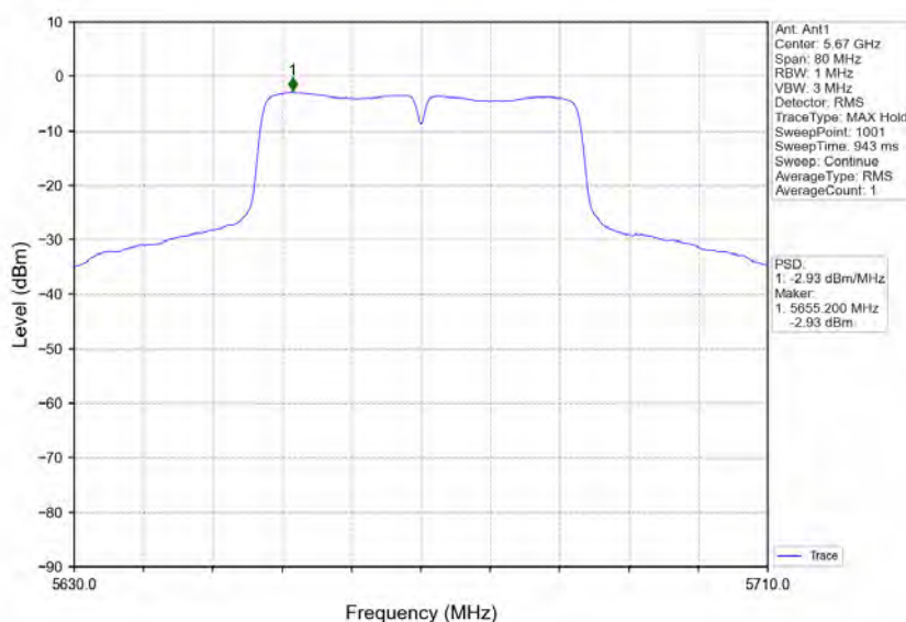
802.11n(HT40)_HCH_5670MHz_Ant1_NTNV
