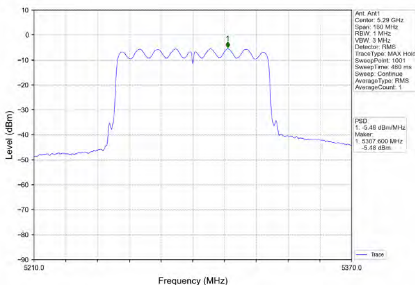
802.11ac(VHT80)_MCH_5290MHz_Ant1_NTNV
