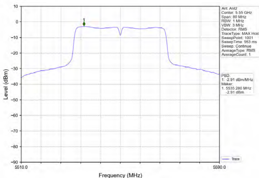
802.11ac(VHT40)_MCH_5550MHz_Ant2_NTNV
