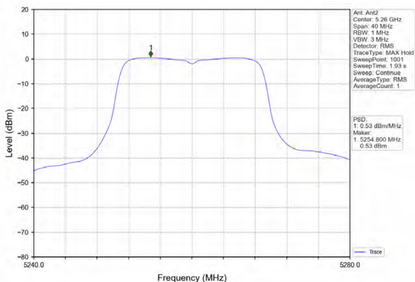
802.11ac(VHT20)_LCH_5260MHz_MIMO_NTNV
