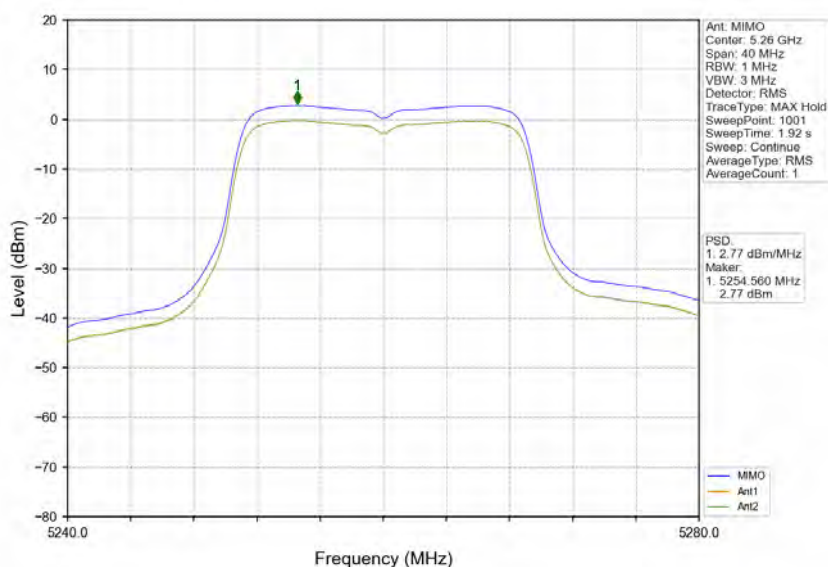
802.11n(HT20)_LCH_5260MHz_MIMO_NTNV
