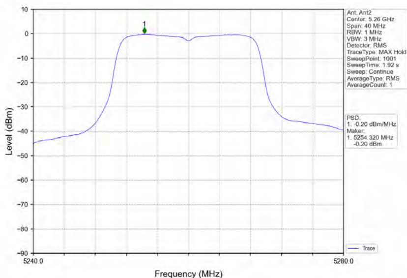
802.11n(HT20)_LCH_5260MHz_MIMO_NTNV
