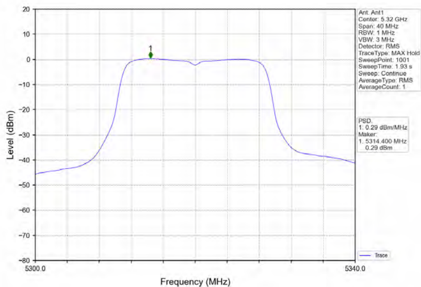
802.11ac(VHT20)_HCH_5320MHz_Ant1_NTNV
