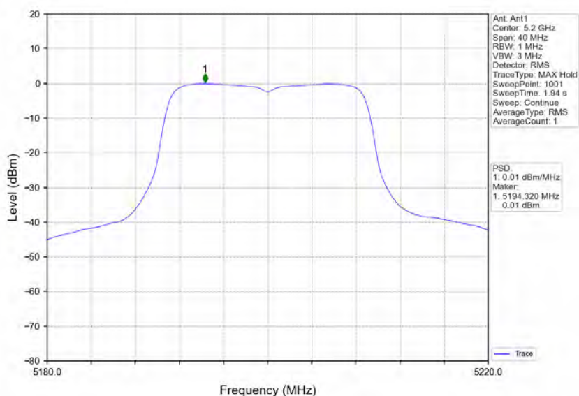
802.11ac(VHT20)_MCH_5200MHz_Ant1_NTNV
