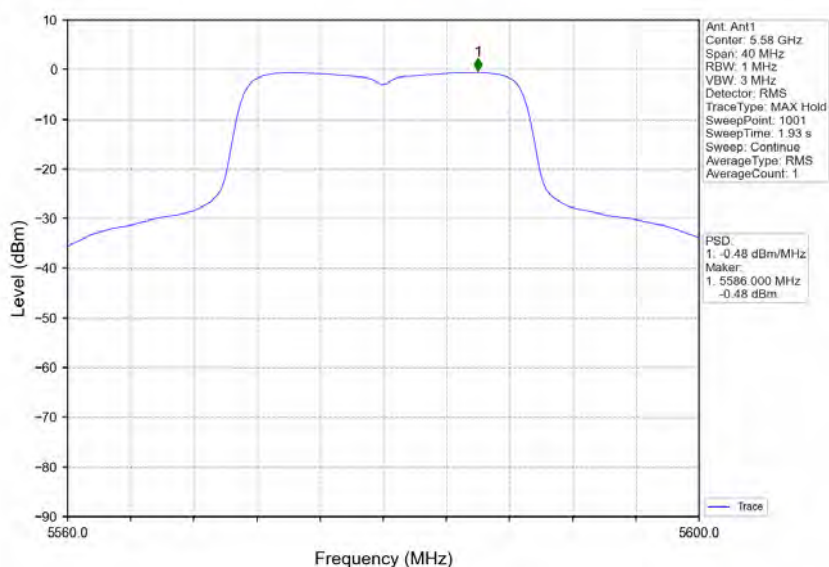
802.11ac(VHT20)_MCH_5580MHz_Ant1_NTNV
