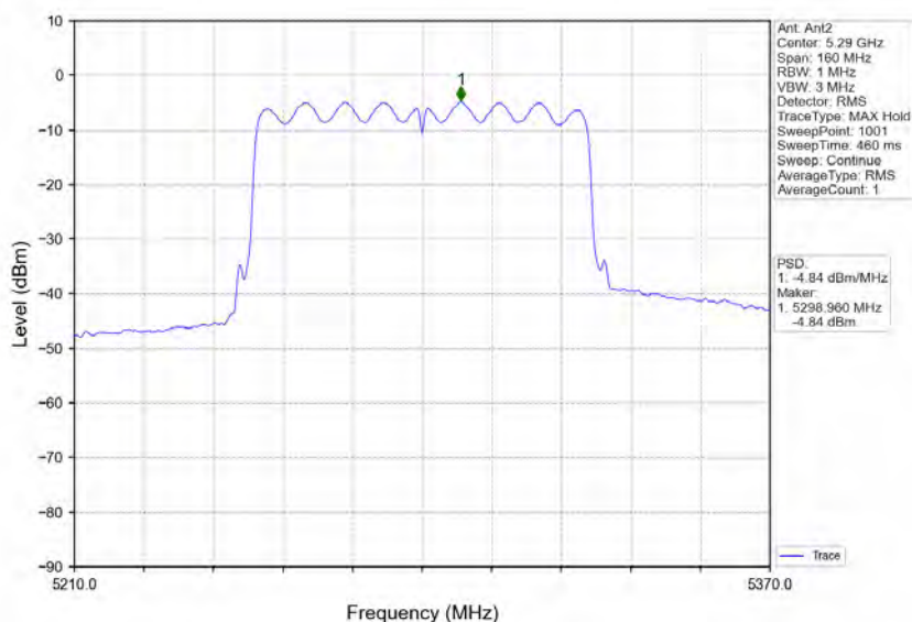
802.11ac(VHT80)_MCH_5290MHz_MIMO_NTNV
