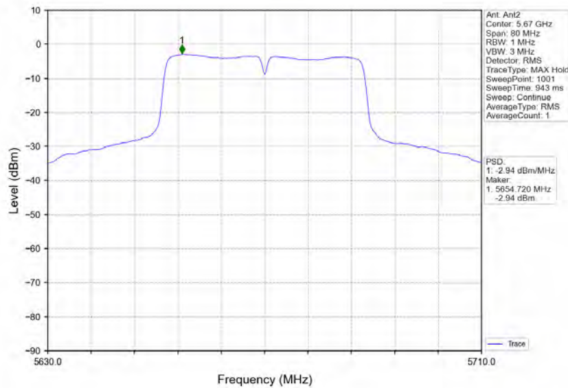
802.11n(HT40)_HCH_5670MHz_MIMO_NTNV
