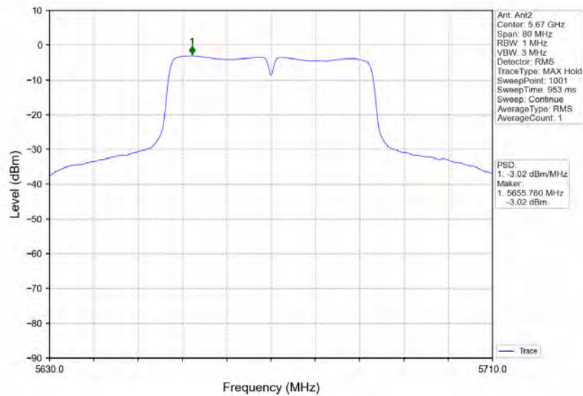
802.11ac(VHT40)_HCH_5670MHz_MIMO_NTNV
