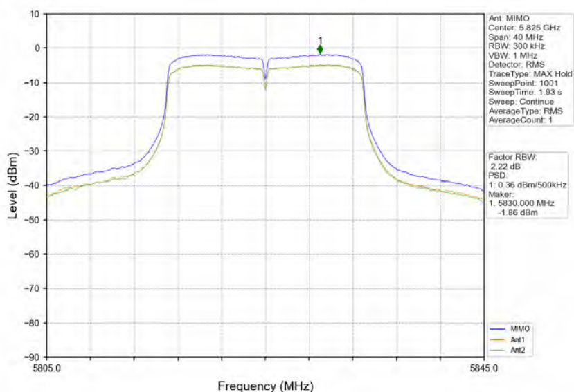
802.11ac(VHT20)_HCH_5825MHz_MIMO_NTNV
