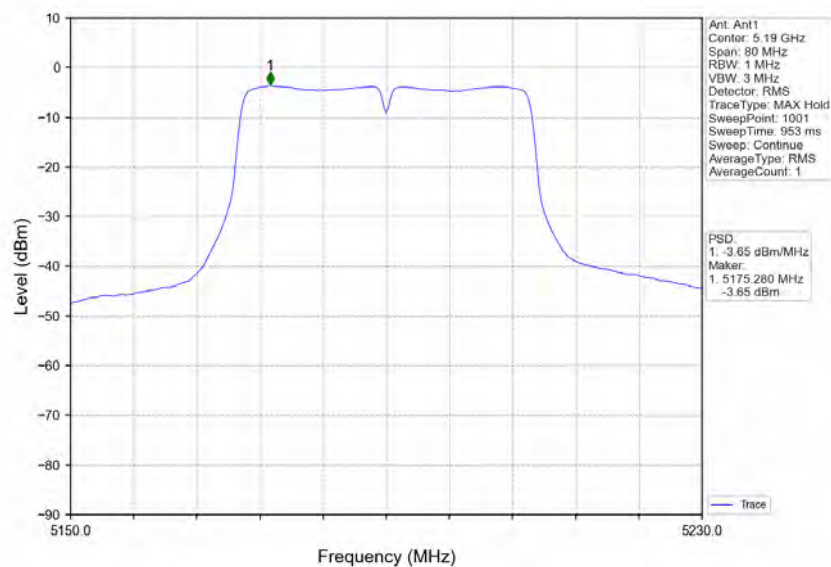
802.11ac(VHT40)_LCH_5190MHz_Ant1_NTNV
