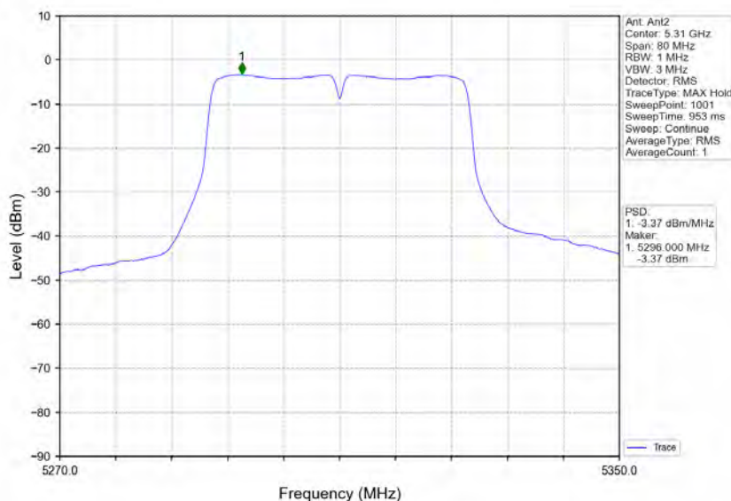
802.11ac(VHT40)_HCH_5310MHz_Ant2_NTNV
