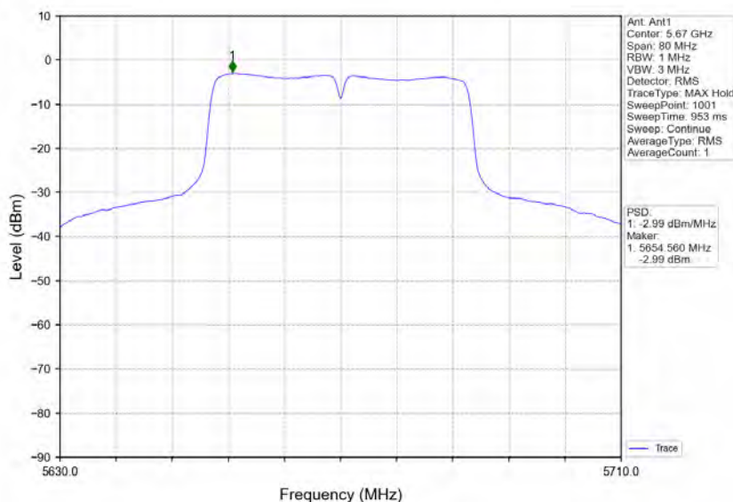
802.11ac(VHT40)_HCH_5670MHz_Ant1_NTNV
