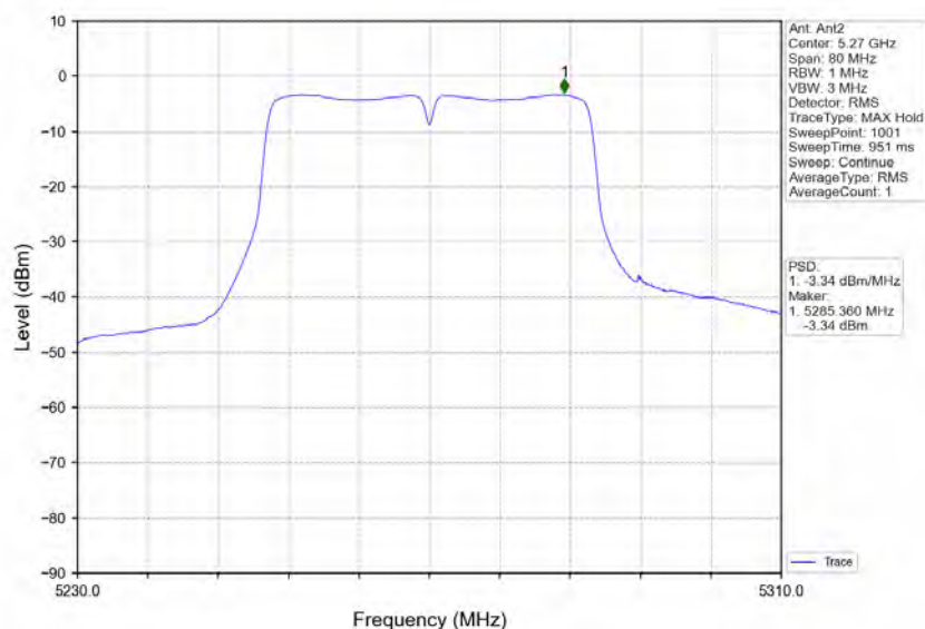
802.11ac(VHT40)_LCH_5270MHz_MIMO_NTNV
