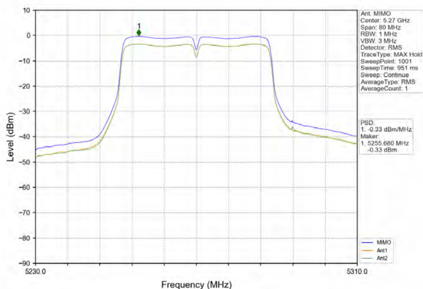
802.11ac(VHT40)_LCH_5270MHz_MIMO_NTNV
