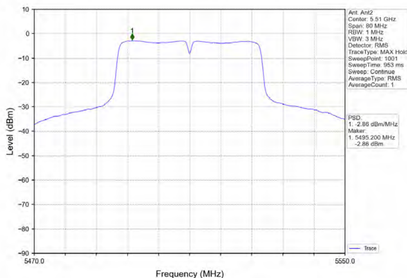
802.11ac(VHT40)_LCH_5510MHz_MIMO_NTNV
