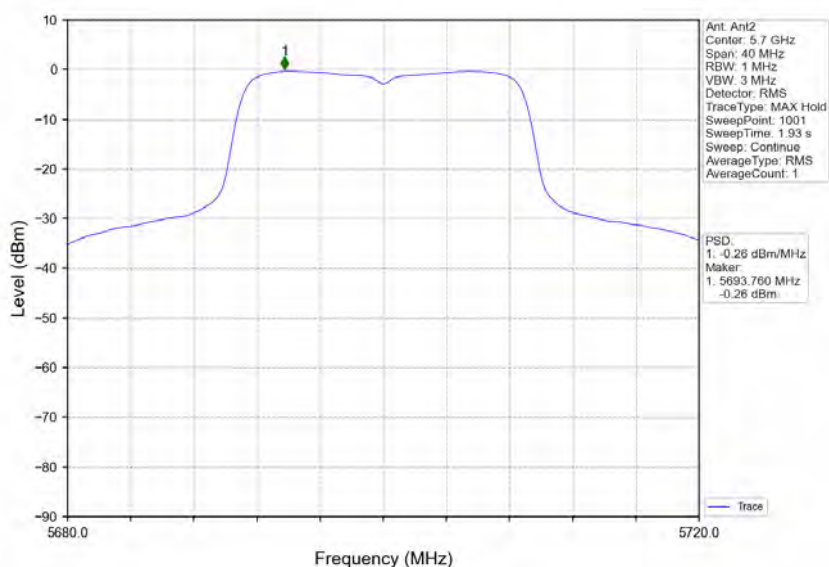
802.11ac(VHT20)_HCH_5700MHz_Ant2_NTNV
