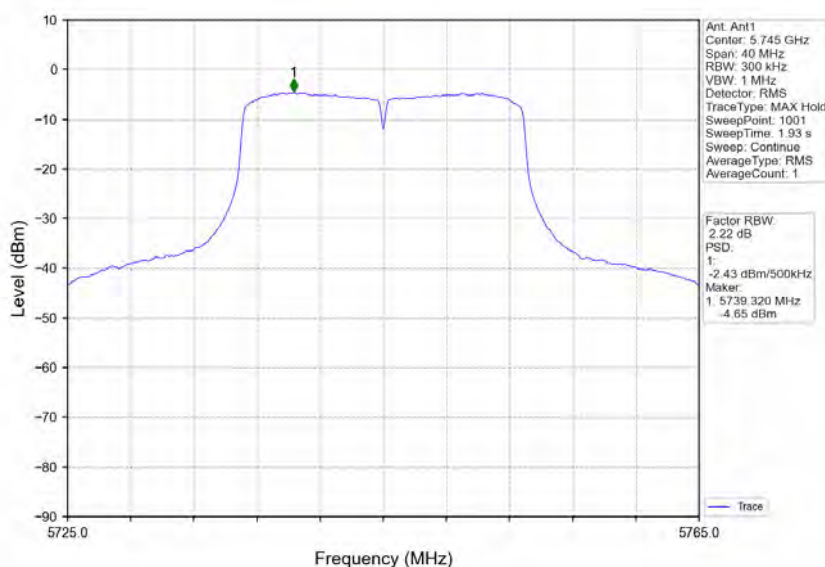
802.11ac(VHT20)_LCH_5745MHz_Ant1_NTNV
