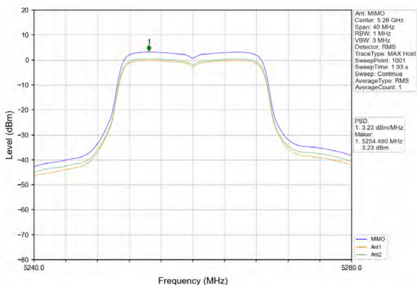
802.11ac(VHT20)_LCH_5260MHz_MIMO_NTNV
