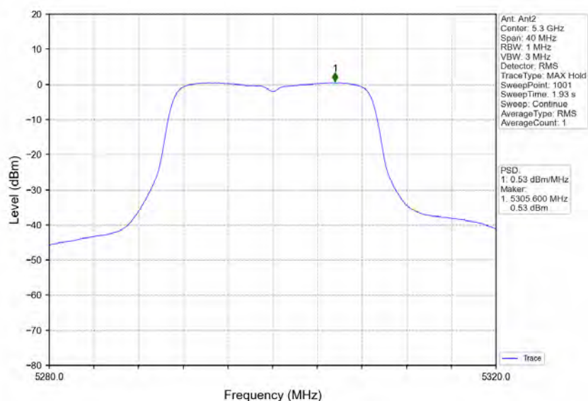
802.11ac(VHT20)_MCH_5300MHz_Ant2_NTNV
