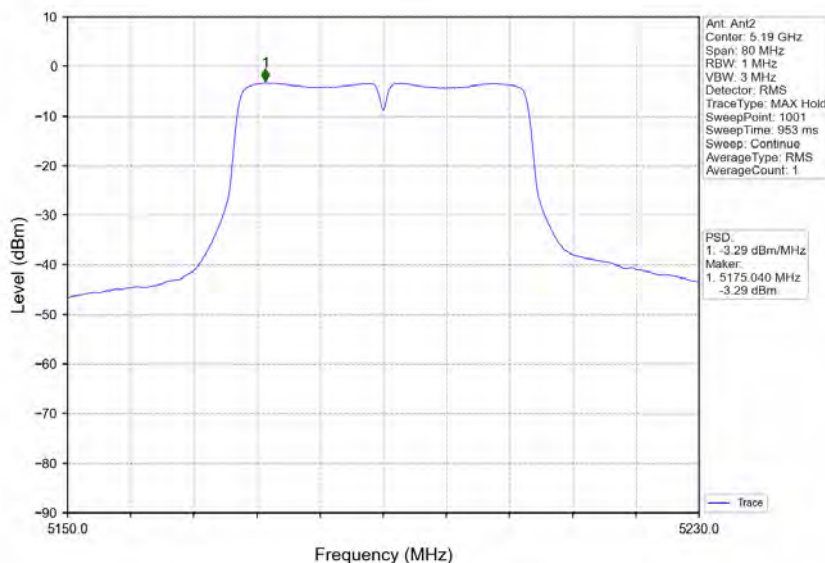
802.11ac(VHT40)_LCH_5190MHz_MIMO_NTNV
