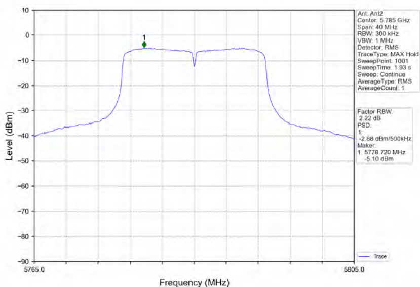
802.11ac(VHT20)_MCH_5785MHz_Ant2_NTNV
