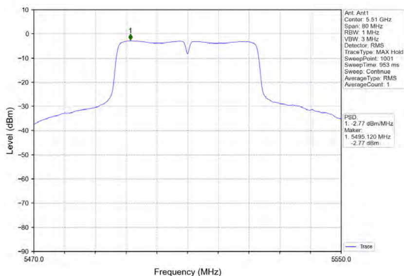
802.11ac(VHT40)_LCH_5510MHz_Ant1_NTNV
