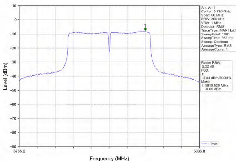
802.11ac(VHT40)_HCH_5795MHz_Ant1_NTNV
