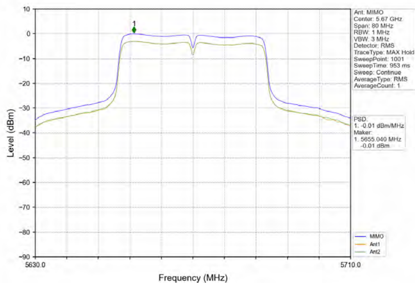
802.11ac(VHT40)_HCH_5670MHz_MIMO_NTNV
