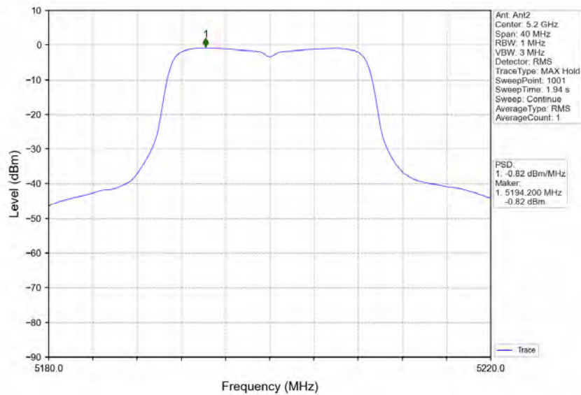
802.11ac(VHT20)_MCH_5200MHz_MIMO_NTNV
