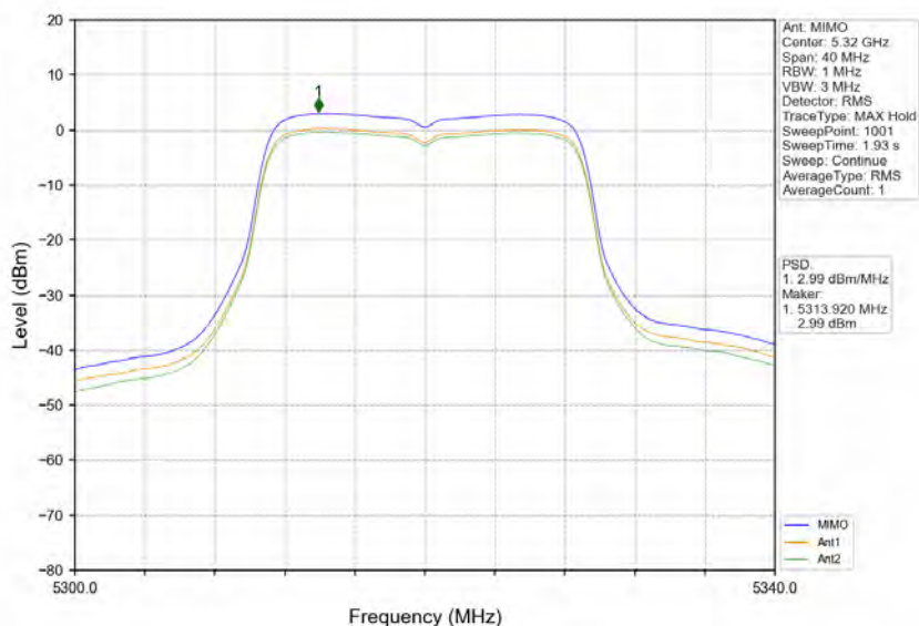
802.11ac(VHT20)_HCH_5320MHz_MIMO_NTNV
