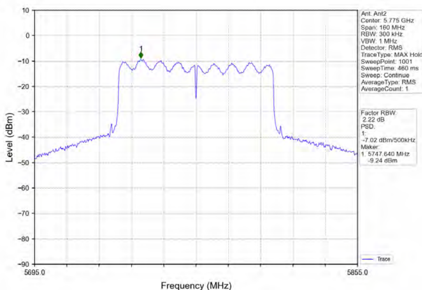
802.11ac(VHT80)_MCH_5775MHz_Ant2_NTNV
