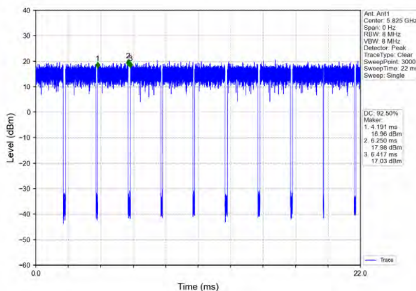
802.11a_HCH_5825MHz_Ant1_NTNV
