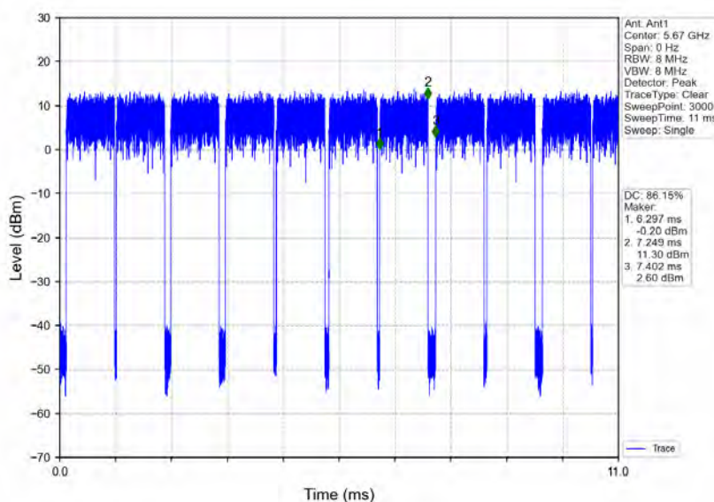
802.11ac(VHT40)_HCH_5670MHz_Ant1_NTNV
