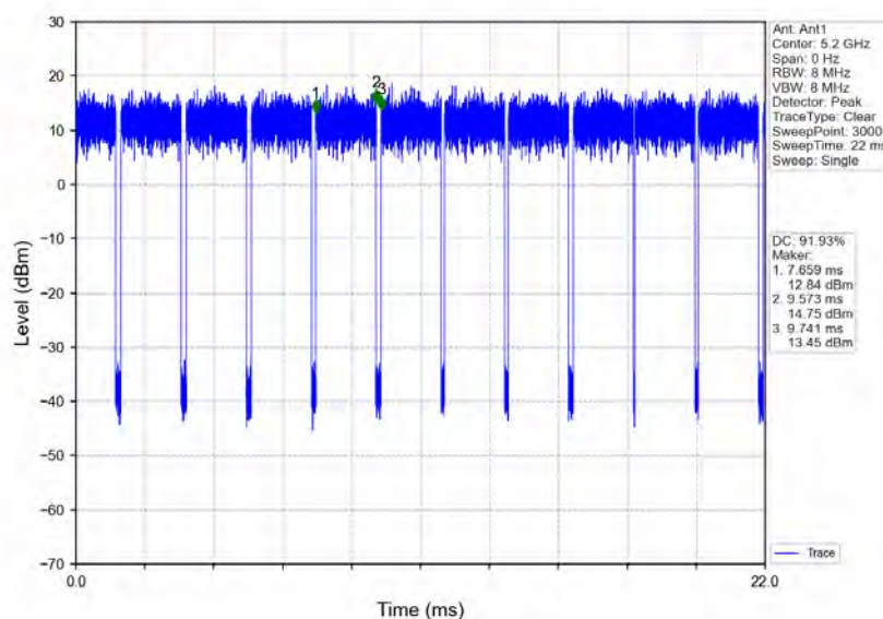
802.11n(HT20)_MCH_5200MHz_Ant1_NTNV
