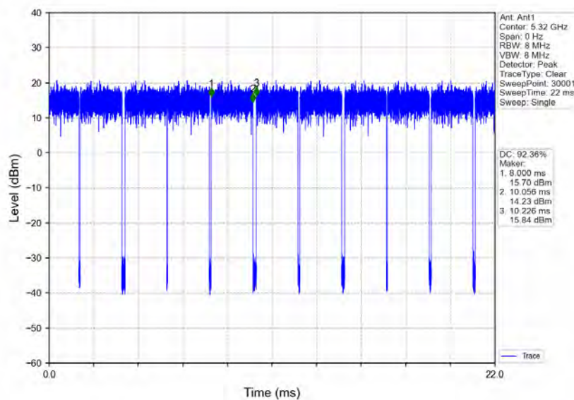
802.11a_HCH_5320MHz_Ant1_NTNV
