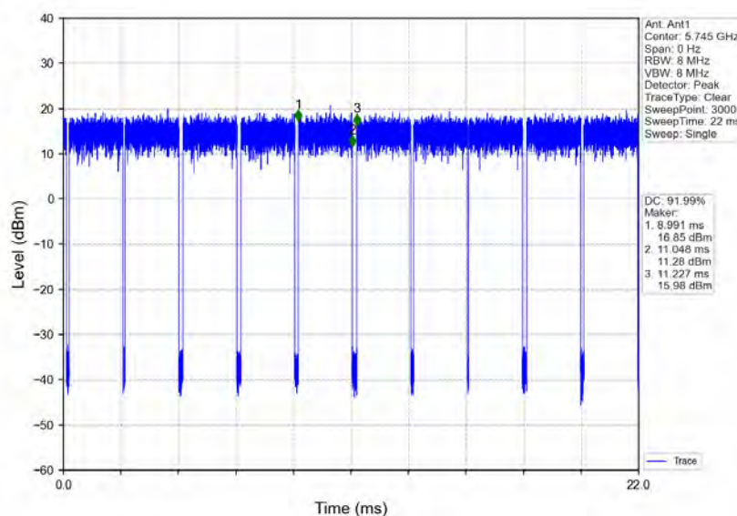
802.11a_LCH_5745MHz_Ant1_NTNV
