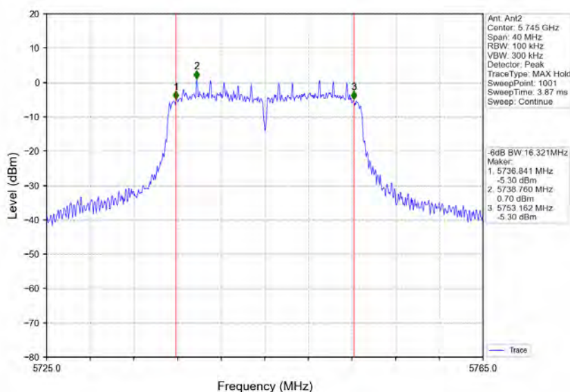
802.11ac(VHT20)_LCH_5745MHz_Ant2_NTNV
