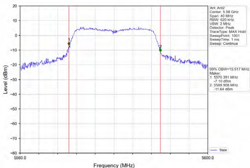
802.11n(HT20)_MCH_5580MHz_Ant2_NTNV
