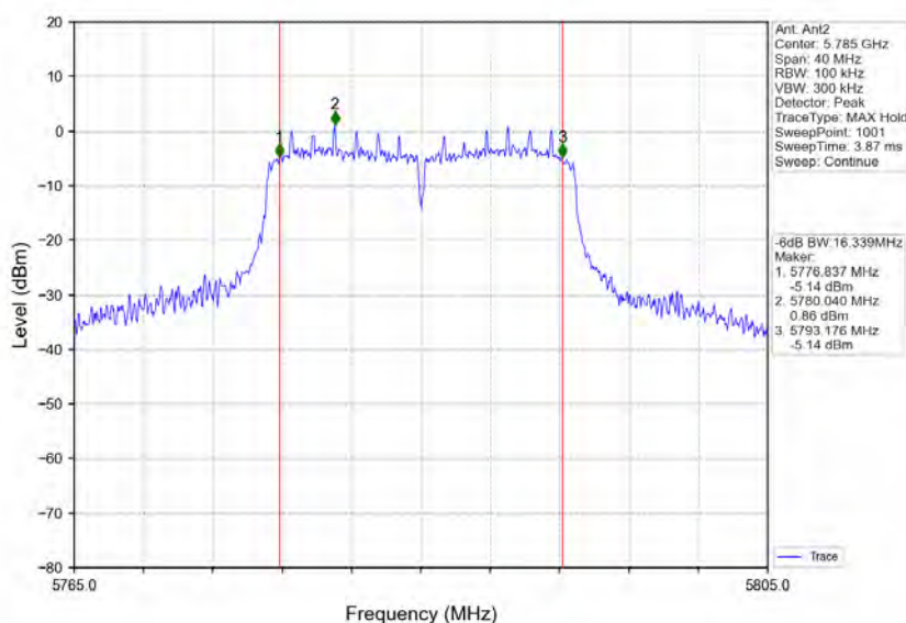
802.11ac(VHT20)_MCH_5785MHz_Ant2_NTNV
