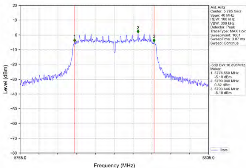
802.11n(HT20)_MCH_5785MHz_Ant2_NTNV
