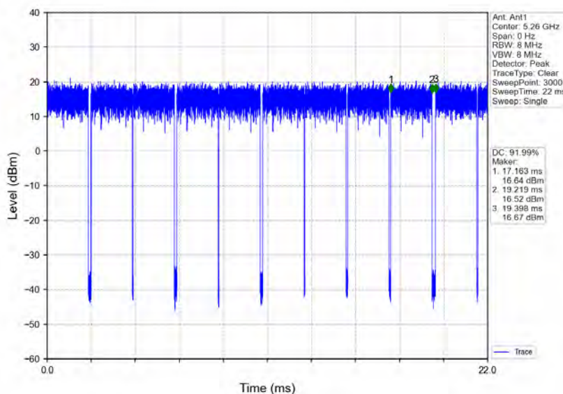
802.11a_LCH_5260MHz_Ant1_NTNV
