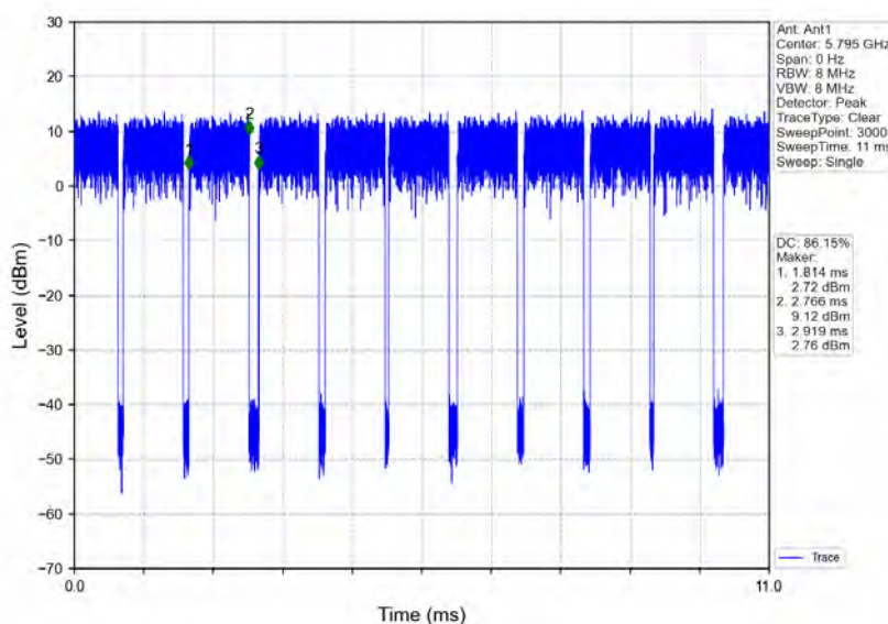
802.11ac(VHT40)_HCH_5795MHz_Ant1_NTNV
