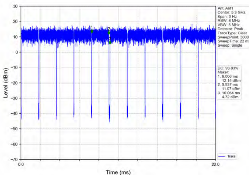
802.11ac(VHT20)_MCH_5300MHz_Ant1_NTNV
