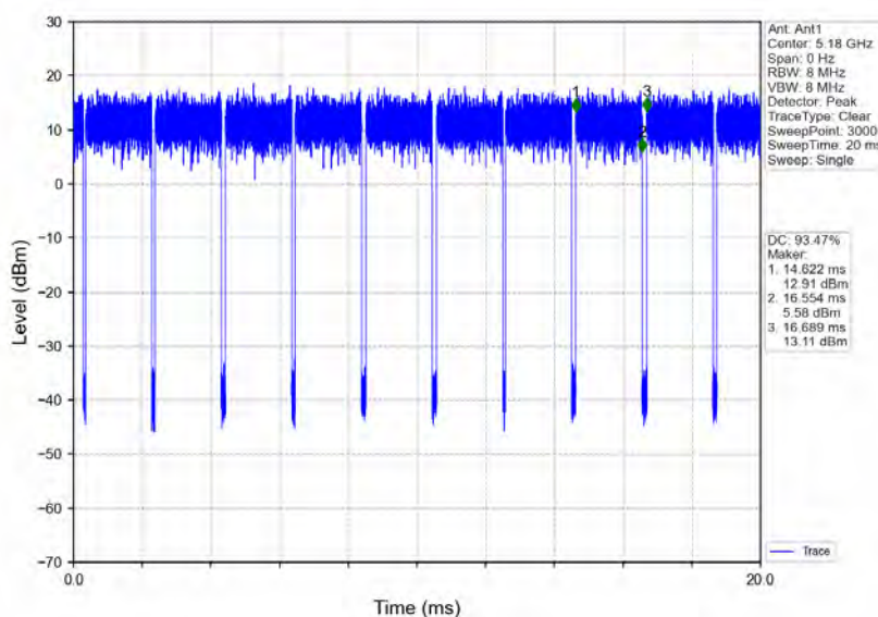
802.11ac(VHT20)_LCH_5180MHz_Ant1_NTNV
