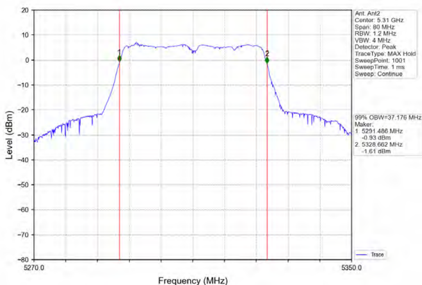
802.11ac(VHT40)_HCH_5310MHz_Ant2_NTNV
