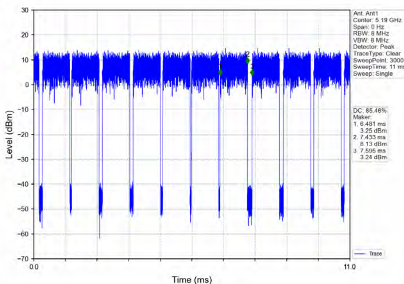
802.11ac(VHT40)_LCH_5190MHz_Ant1_NTNV
