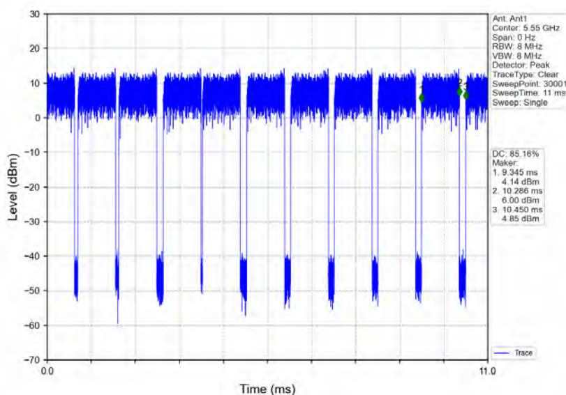
802.11n(HT40)_MCH_5550MHz_Ant1_NTNV
