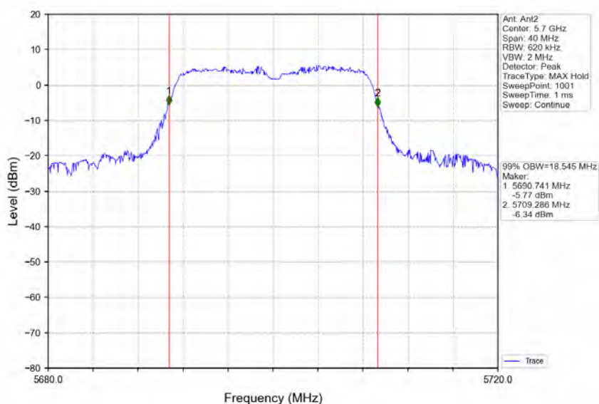
802.11ac(VHT20)_HCH_5700MHz_Ant2_NTNV
