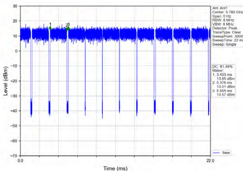
802.11ac(VHT20)_MCH_5785MHz_Ant1_NTNV
