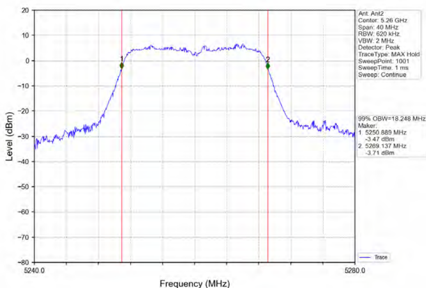
802.11ac(VHT20)_LCH_5260MHz_Ant2_NTNV
