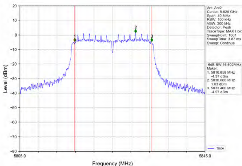
802.11ac(VHT20)_HCH_5825MHz_Ant2_NTNV
