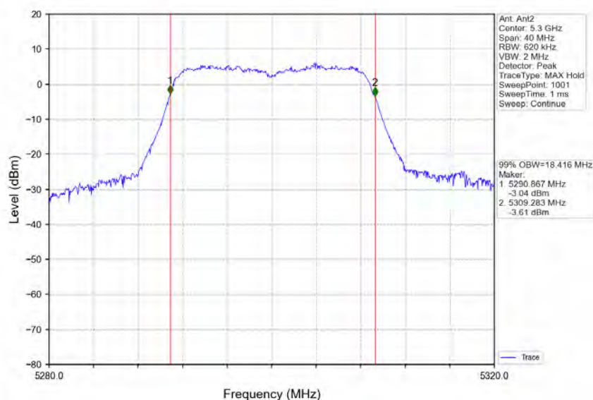
802.11ac(VHT20)_MCH_5300MHz_Ant2_NTNV
