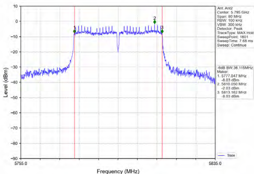
802.11ac(VHT40)_HCH_5795MHz_Ant2_NTNV
