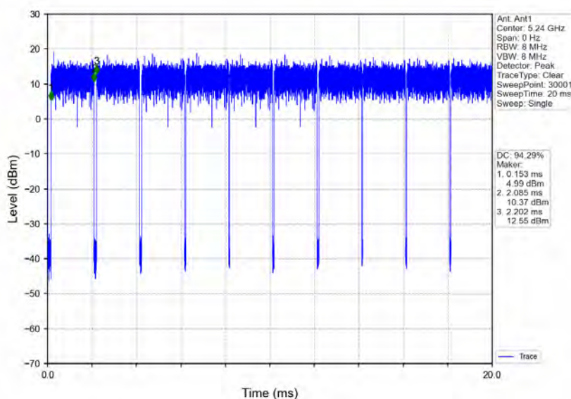
802.11ac(VHT20)_HCH_5240MHz_Ant1_NTNV
