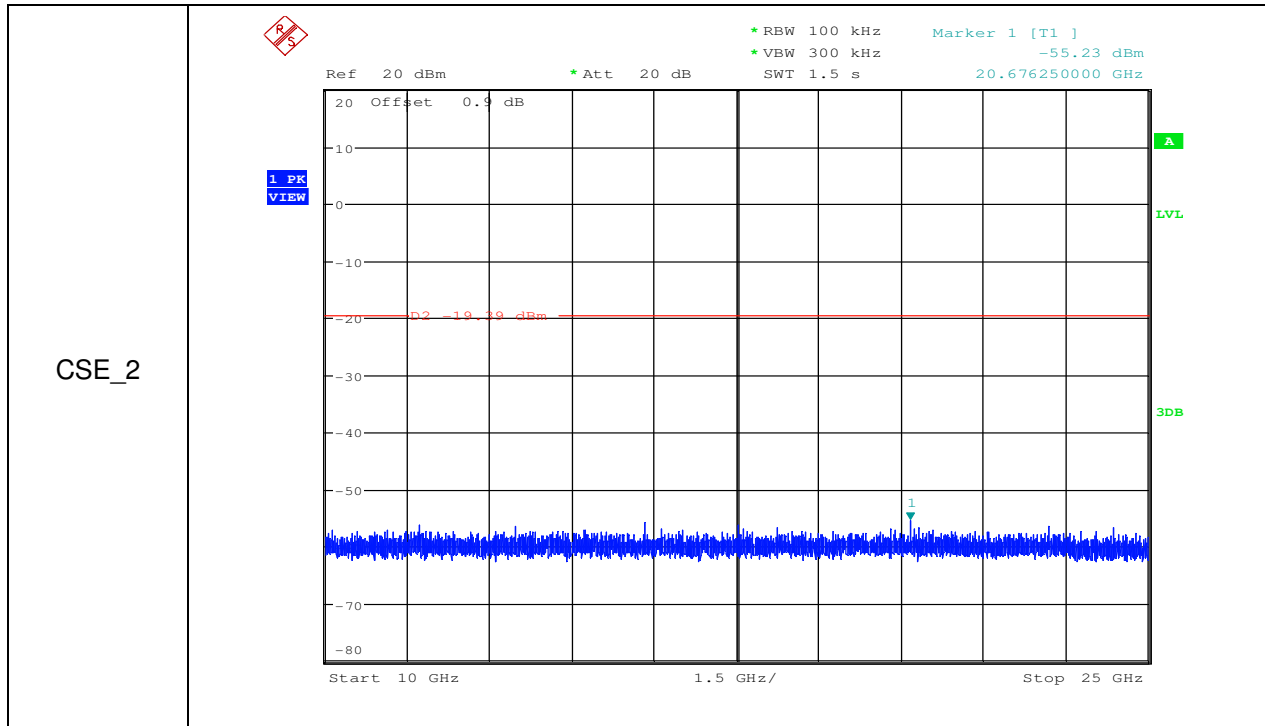
RF Conducted Spurious Emissions_11G_2462_Ant2
