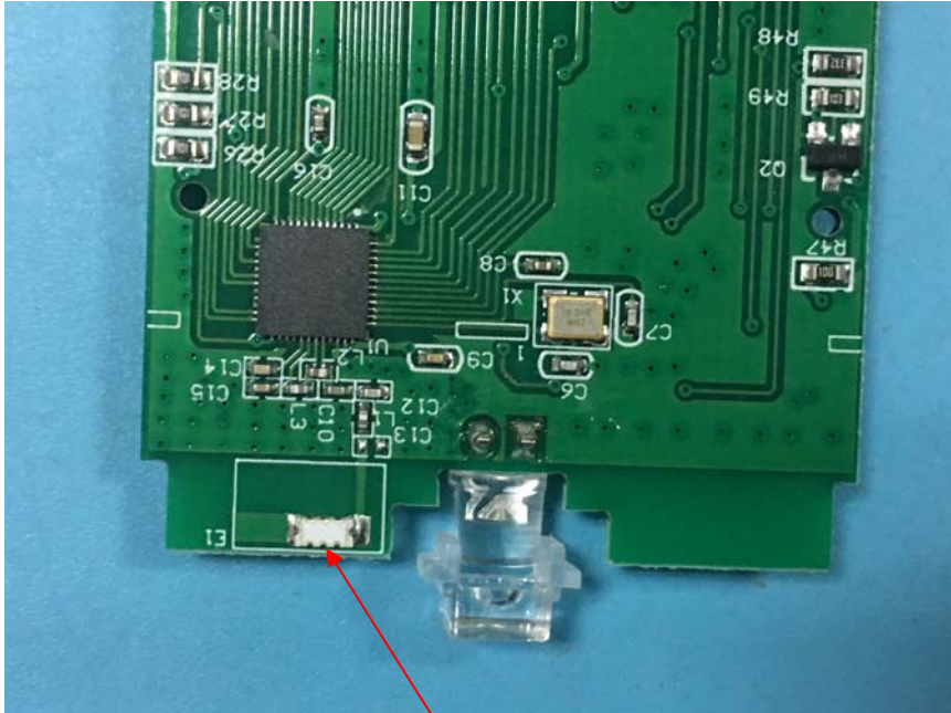
TX Antenna
